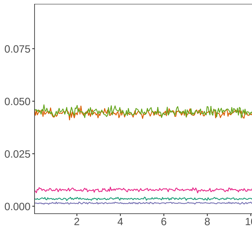
Methionine
