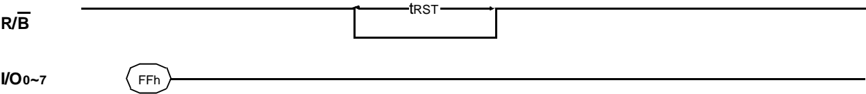
Figure 23. RESET Operation
