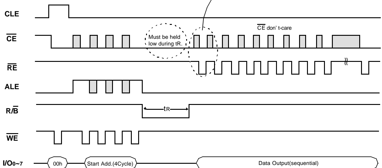
Figure 7. Read Operation with \overline{CE} don't t-care.
