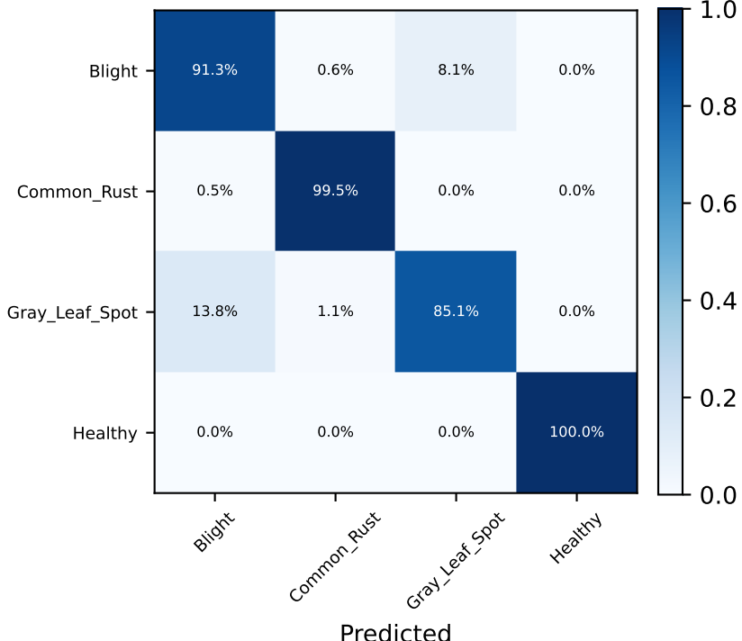
corn maize leaf disease — baseline (normalized)
