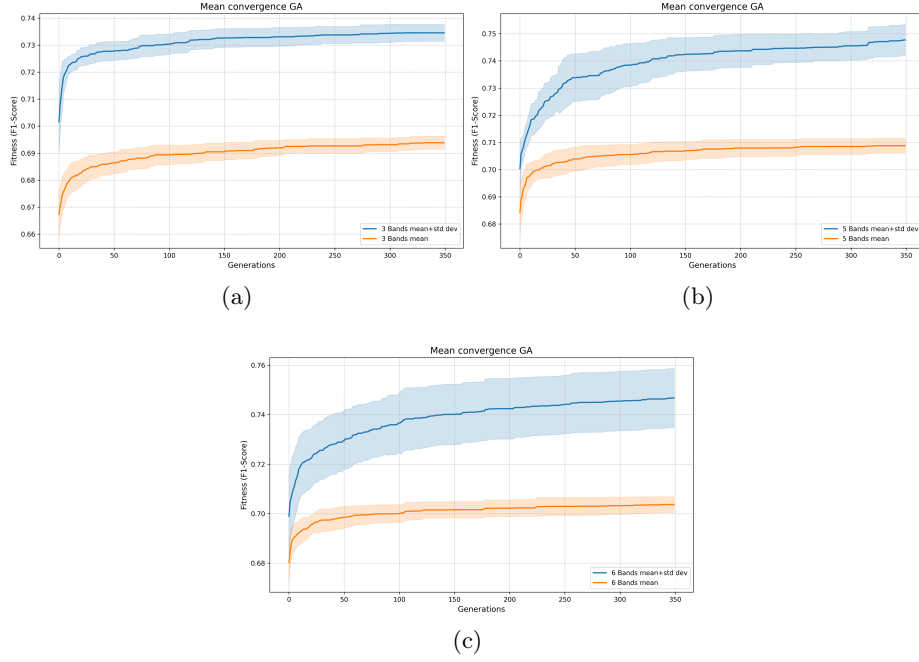
Fig. 4: Genetic Algorithm convergence profiles: (a) 3-band; (b) 5-band; and (c) 6-band optimization scenarios.
