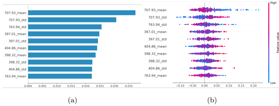
Fig. 7: Global explainability analysis (SHAP) for the optimal GA 5 band model. (a) Mean absolute feature importance ranking. (b) Beeswarm summary plot illustrating feature impact and directionality on the infected class.
