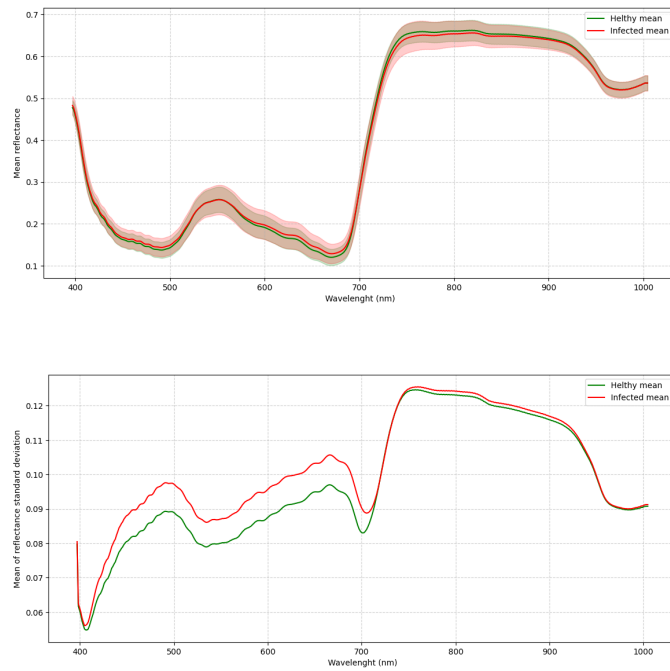
FIGURE 3 | Spectral characterization of the fig samples. (a) Average reflectance signatures. (b) Standard deviation signatures.
