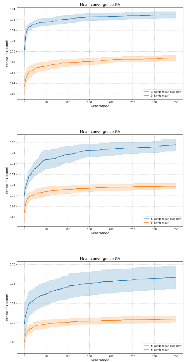
FIGURE 4 | Genetic Algorithm convergence profiles: (a) 3-band; (b) 5-band; and (c) 6-band optimization scenarios.
