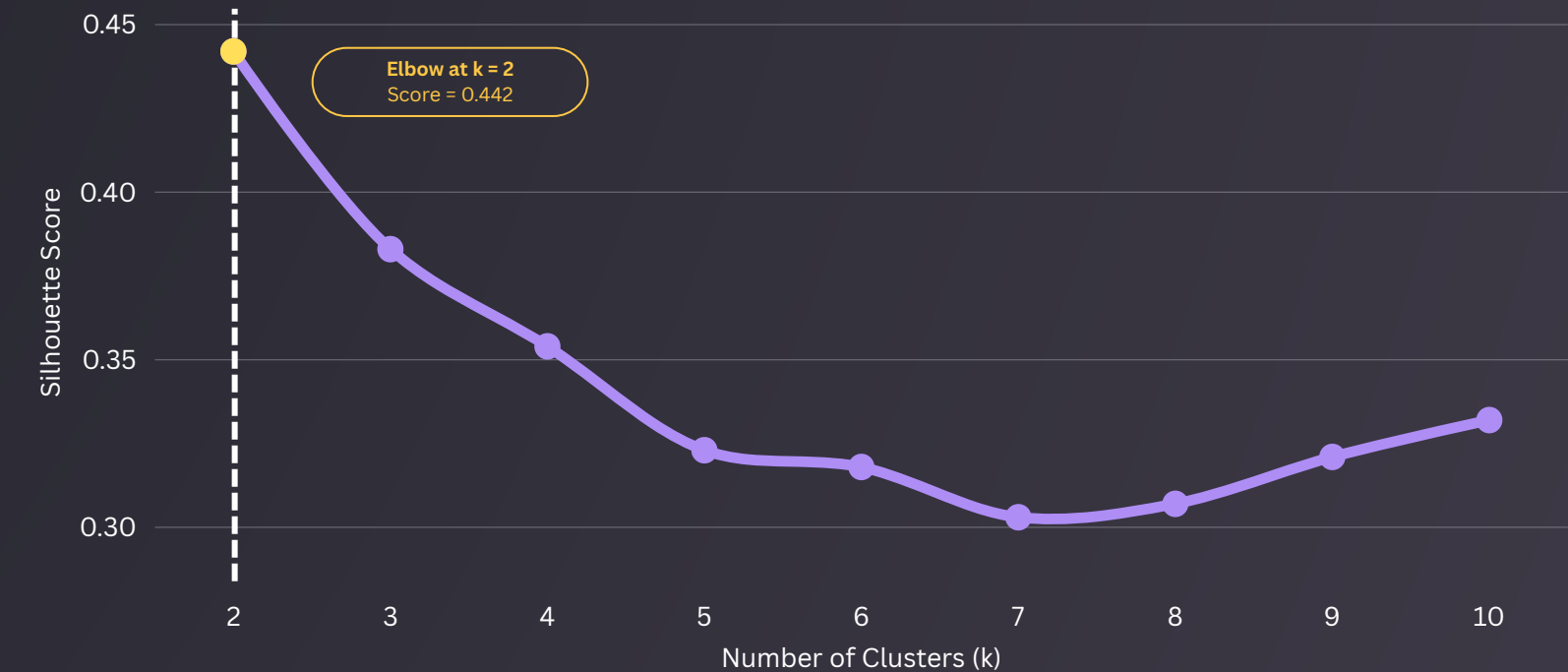
Silhouette Score Analysis for KMeans Clustering
