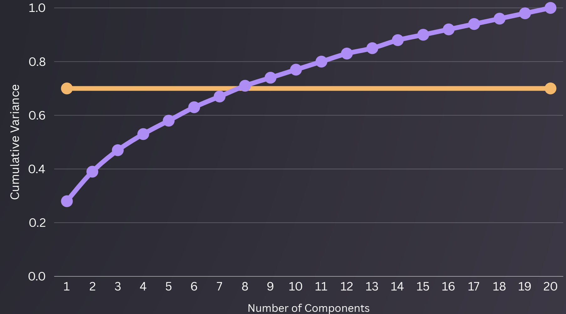
PCA - Cumulative Explained Variance
