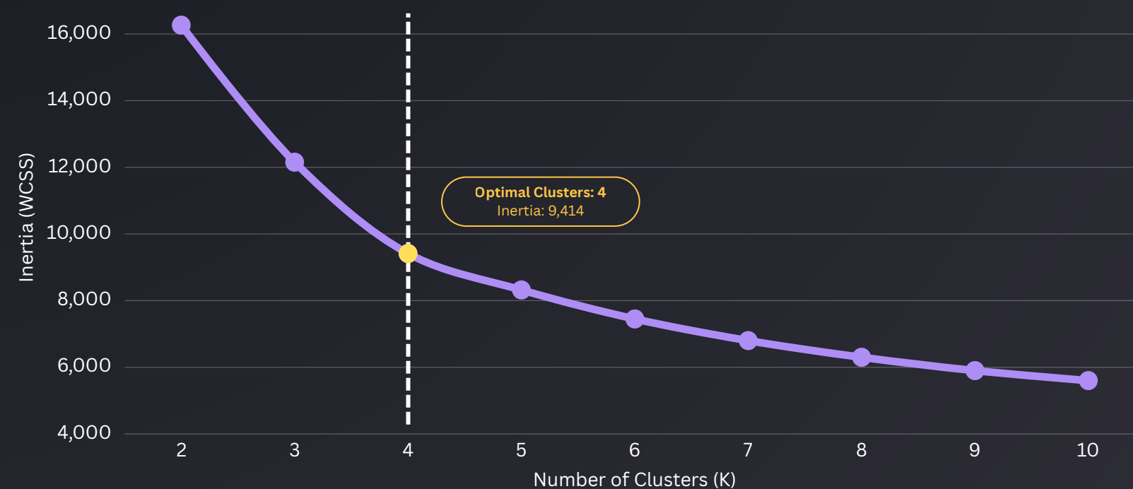
Elbow Method for Optimal K
