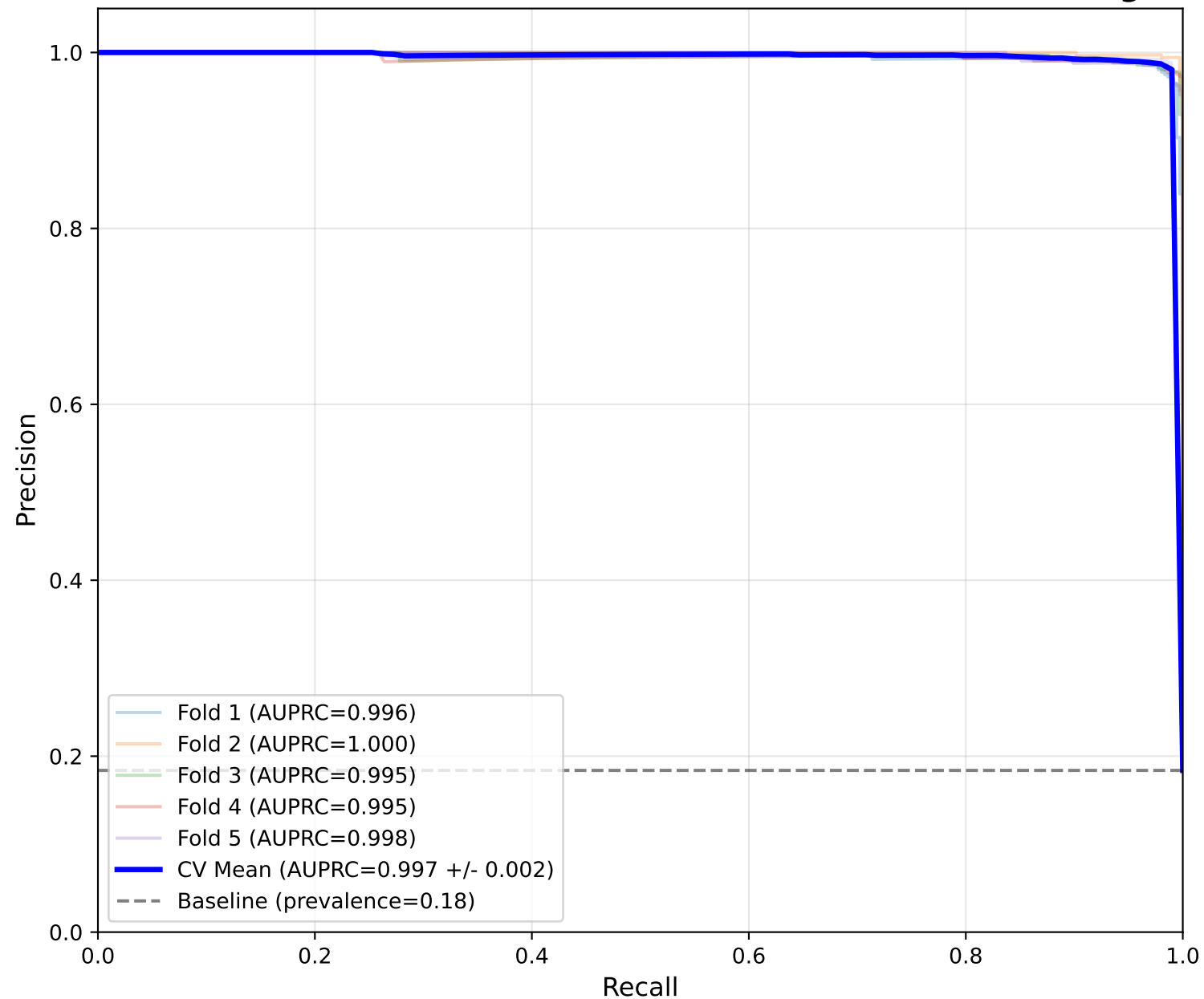
Precision-Recall Curves - 5-Fold CV (12-Lead, No Windowing)
