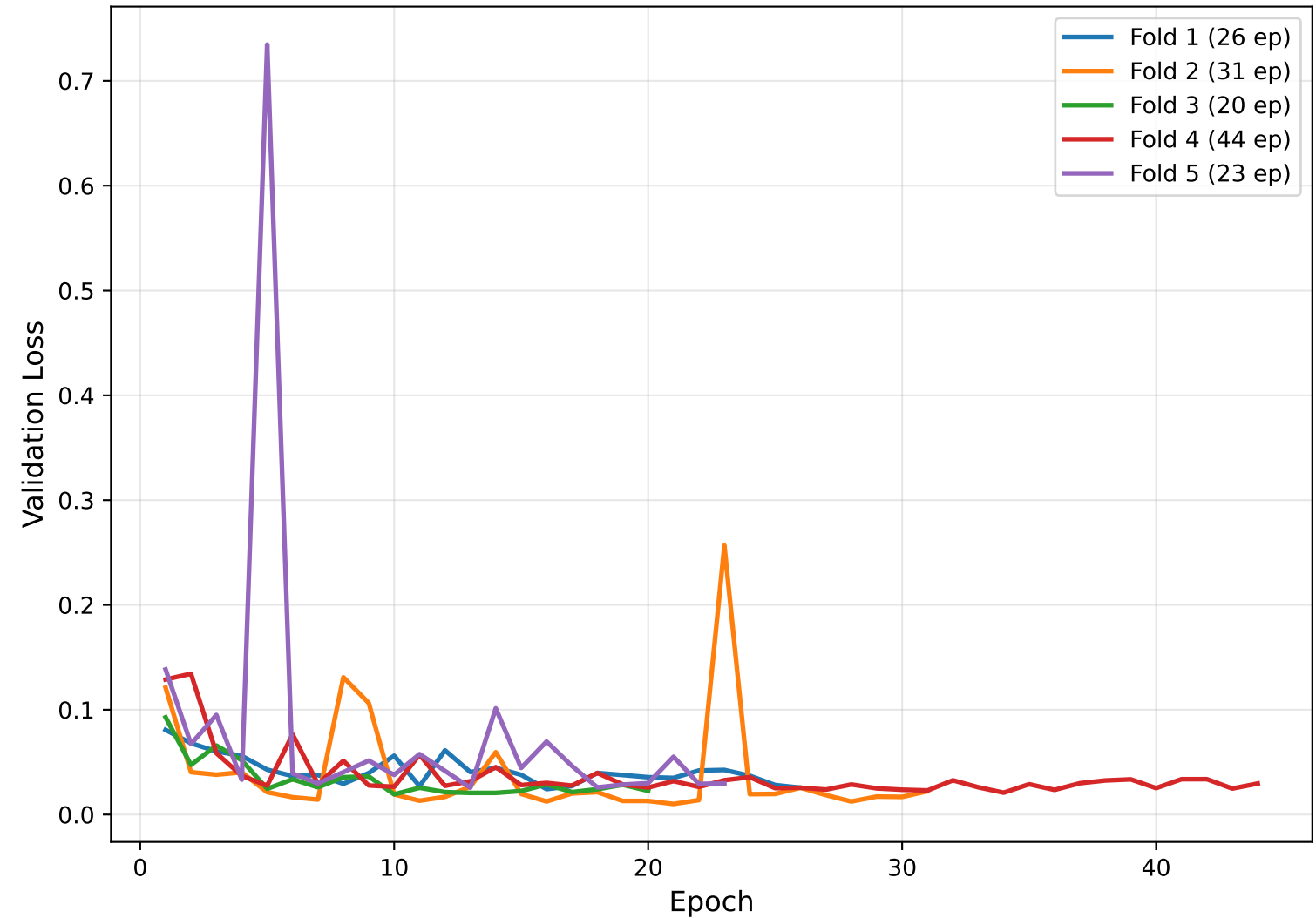
Validation Loss - 5-Fold CV (12-Lead, No Windowing)
