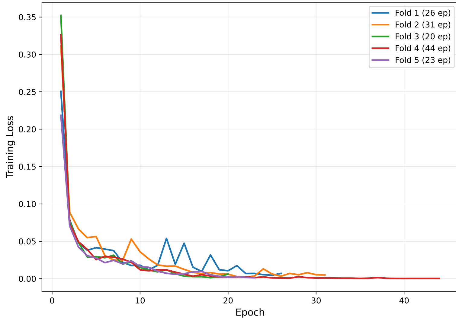
Training Loss - 5-Fold CV (12-Lead, No Windowing)
