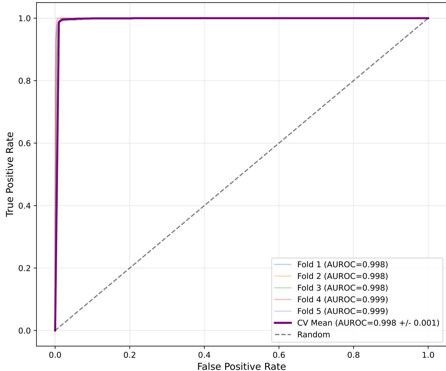
ROC Curves - CNN-BiLSTM (5-Fold CV)
