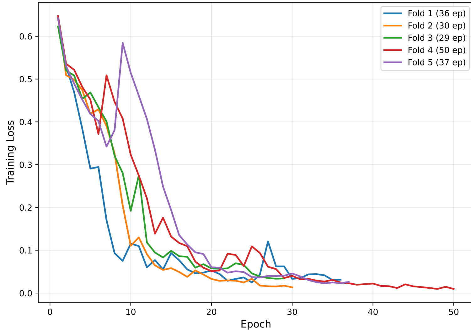
Training Loss - CNN-BiLSTM (5-Fold CV)
