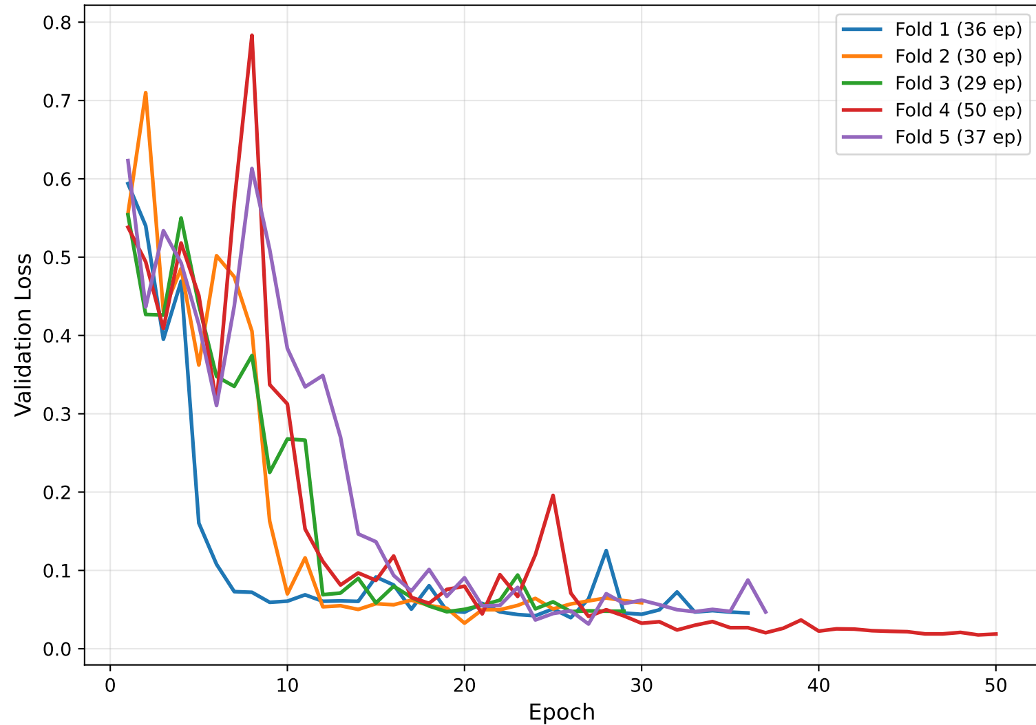
Validation Loss - CNN-BiLSTM (5-Fold CV)
