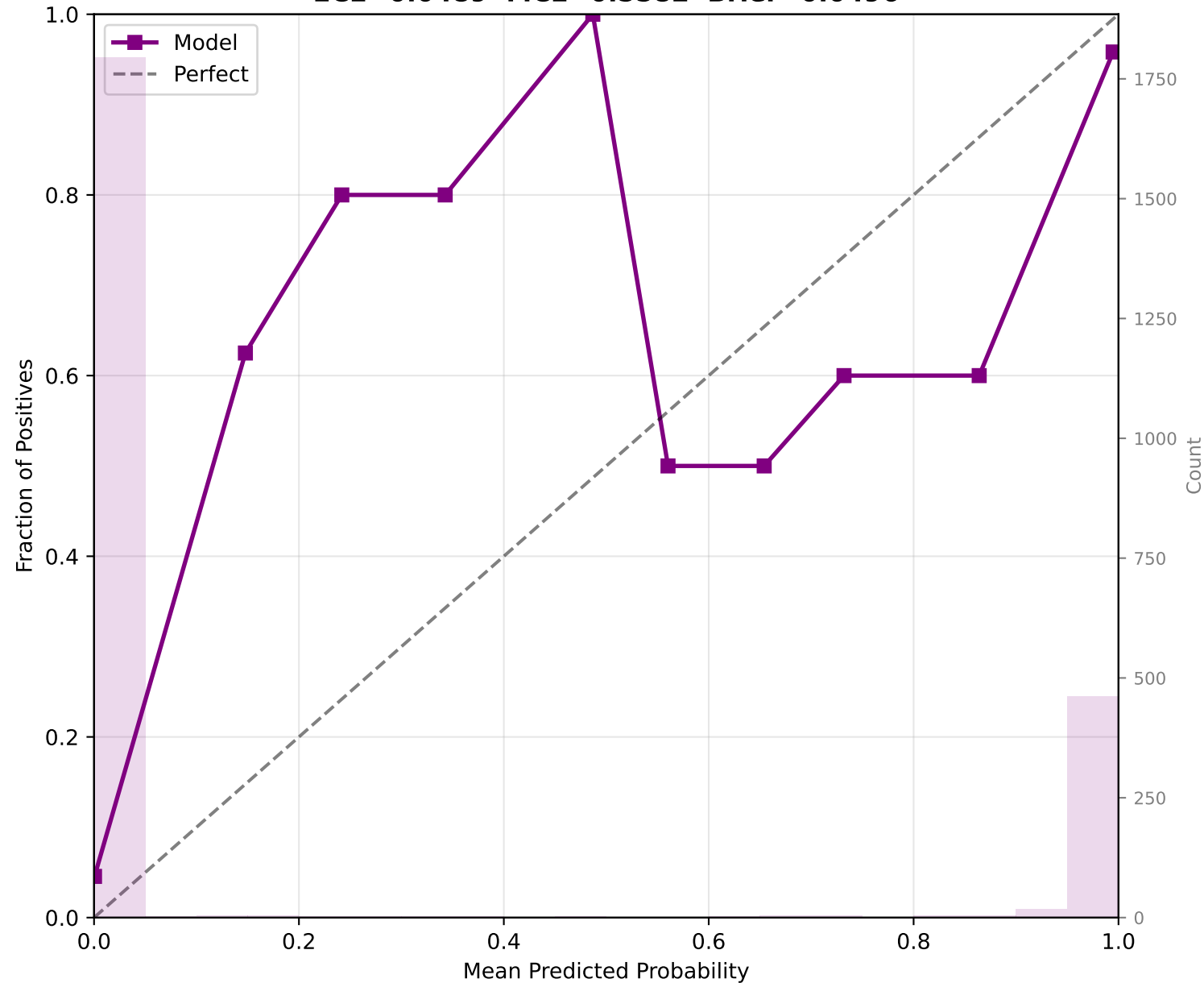
Calibration — CNN-BiLSTM Cross-Dataset (Chapman-Shaoxing → Georgia) ECE=0.0489 MCE=0.5582 Brier=0.0496
