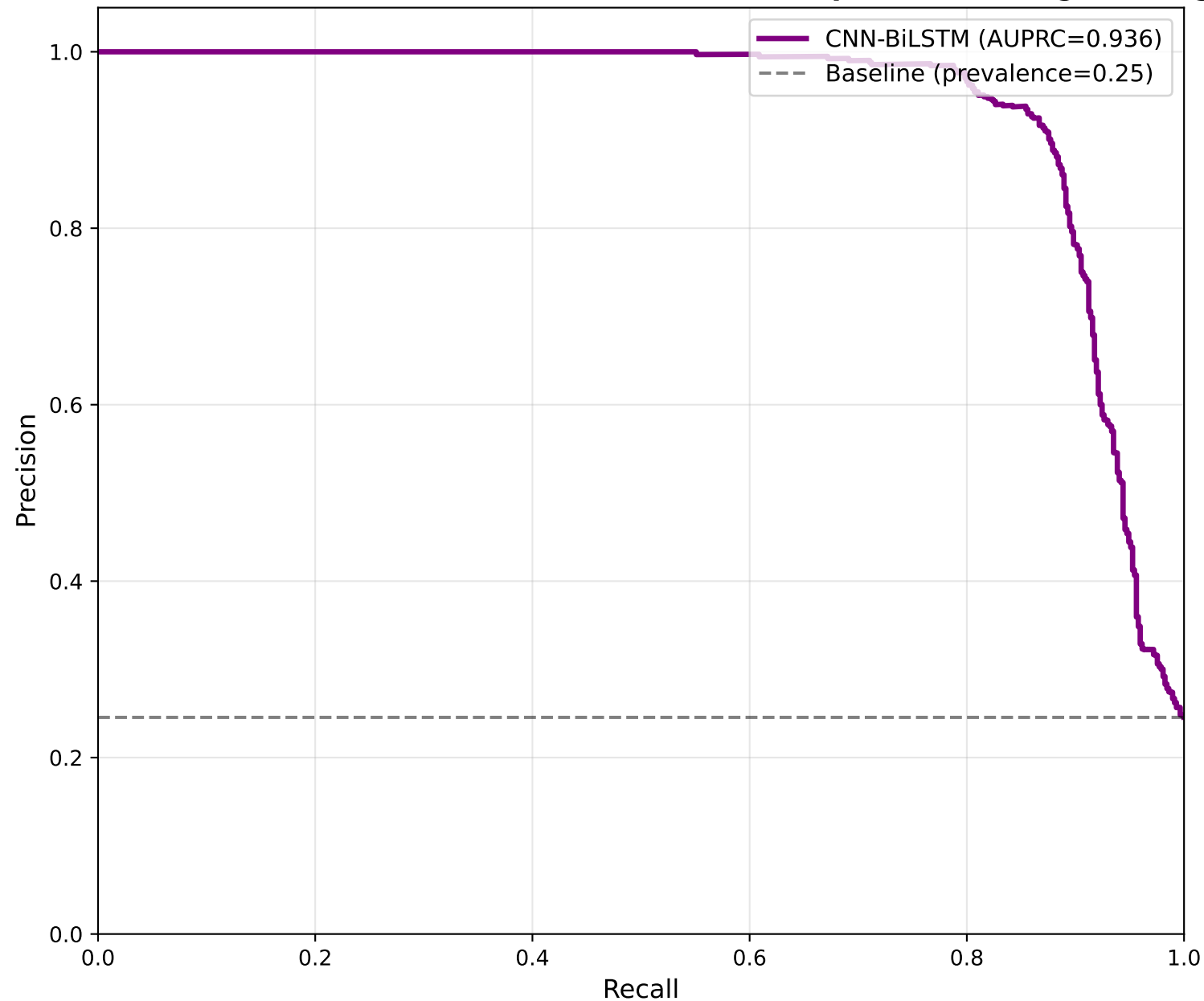
Precision-Recall — CNN-BiLSTM Cross-Dataset (Chapman-Shaoxing → Georgia)
