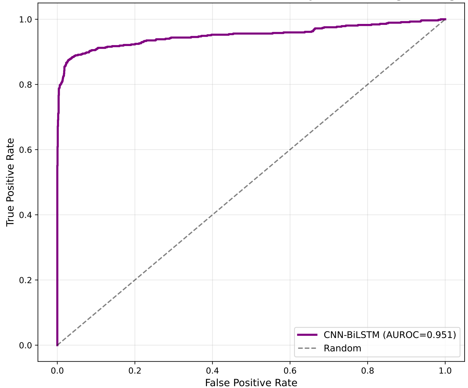
ROC Curve — CNN-BiLSTM Cross-Dataset (Chapman-Shaoxing → Georgia)
