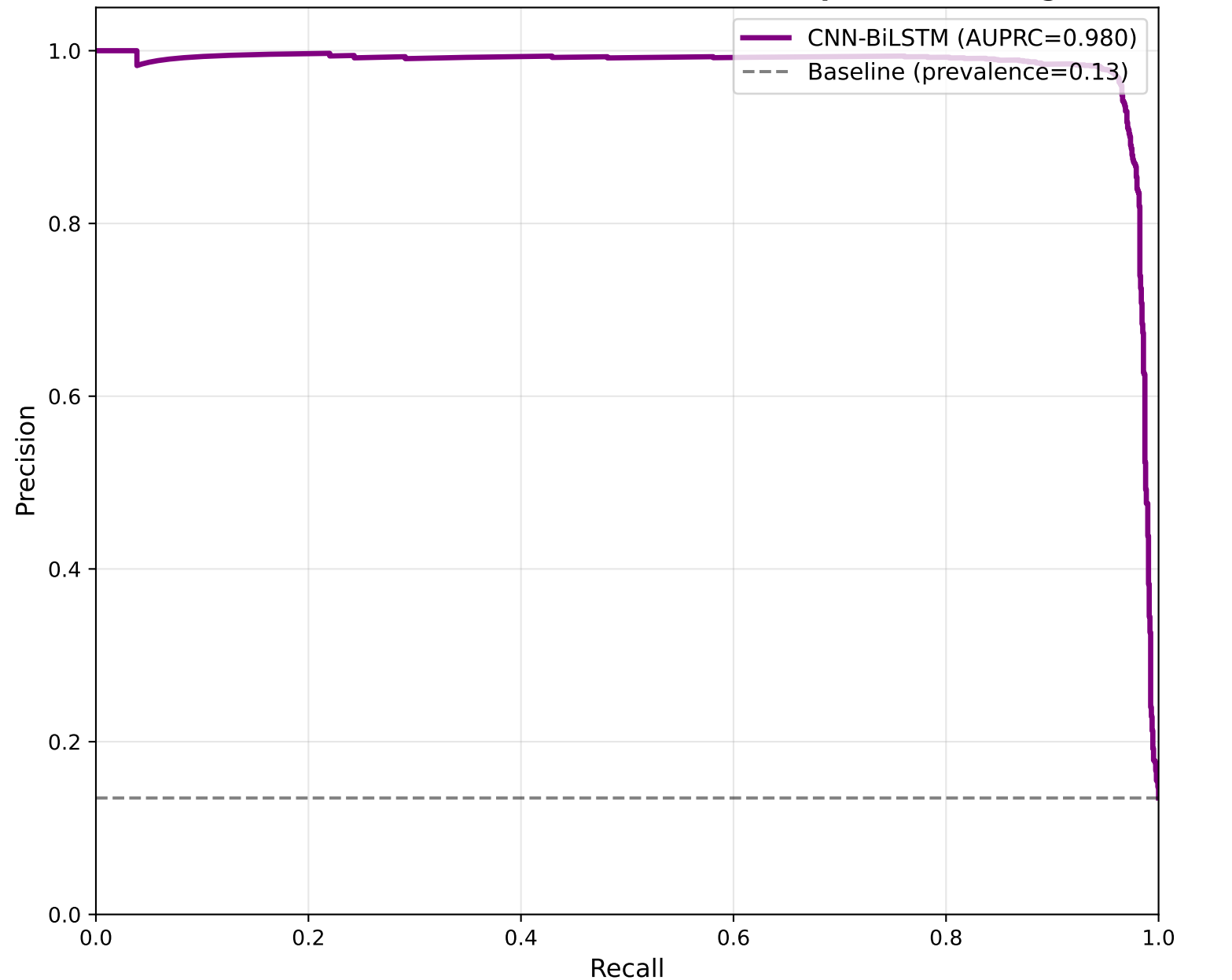
Precision-Recall — CNN-BiLSTM Cross-Dataset (Chapman-Shaoxing → PTB-XL)
