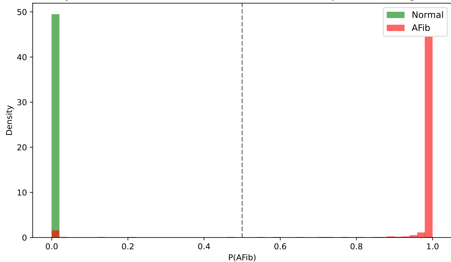
Probability Distribution — CNN-BiLSTM Cross-Dataset (Chapman-Shaoxing → PTB-XL)
