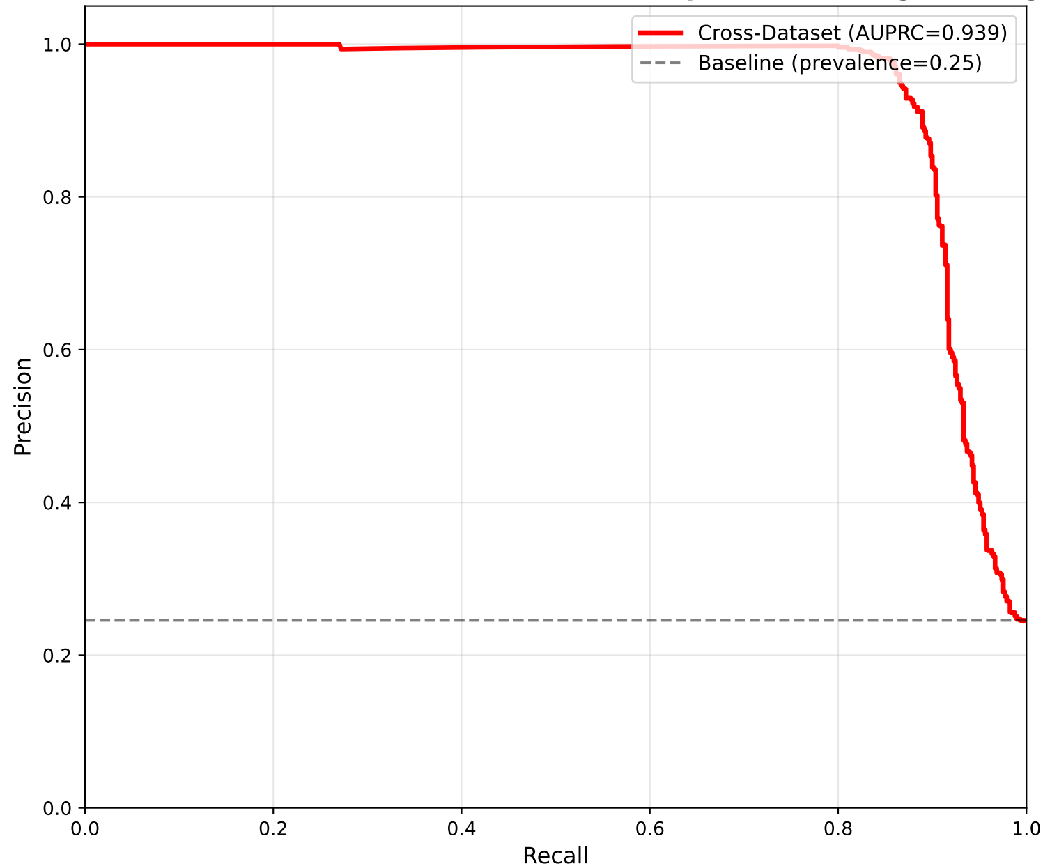
Precision-Recall Curve — Cross-Dataset (Chapman-Shaoxing → Georgia)
