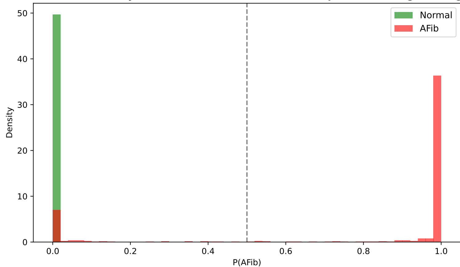
Predicted Probability Distribution — Cross-Dataset (Chapman-Shaoxing → Georgia)
