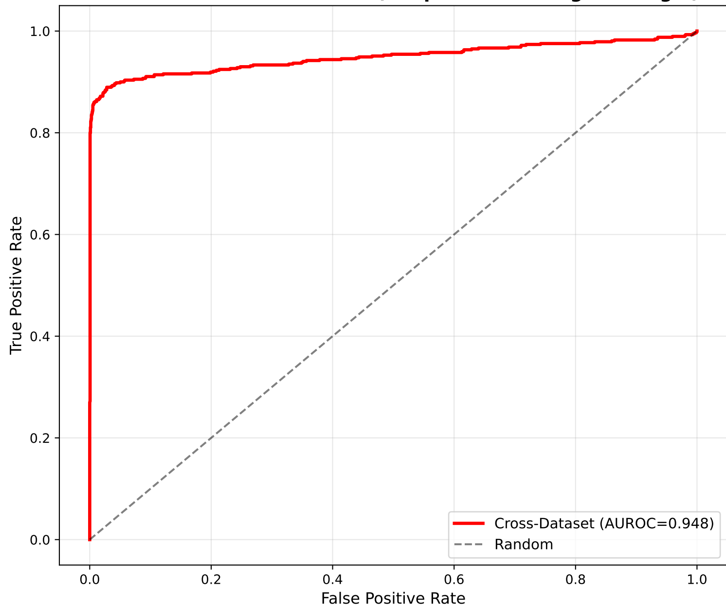
ROC Curve — Cross-Dataset (Chapman-Shaoxing → Georgia)
