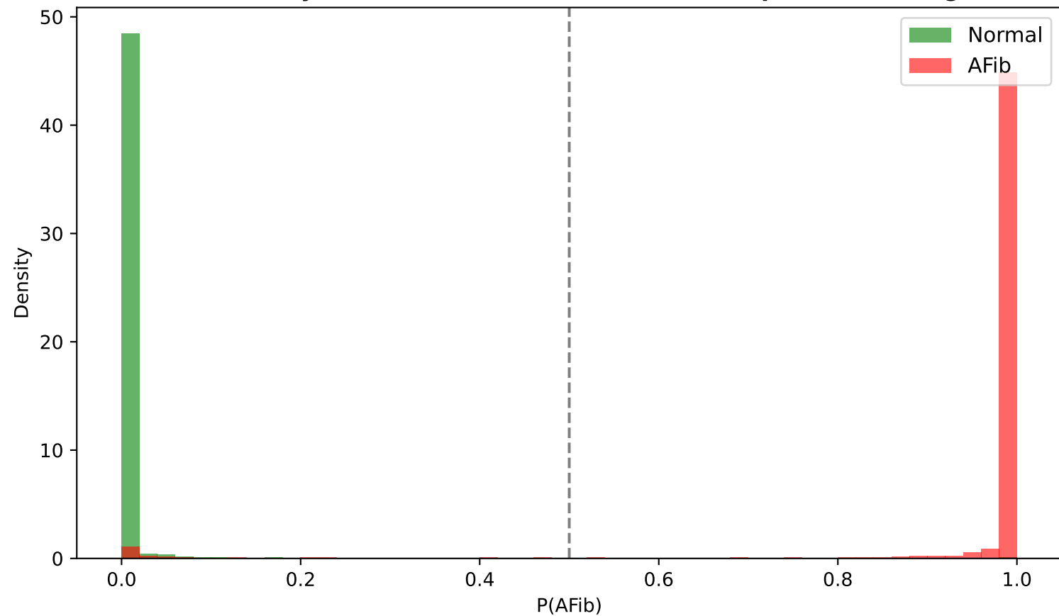
Predicted Probability Distribution — Cross-Dataset (Chapman-Shaoxing → PTB-XL)
