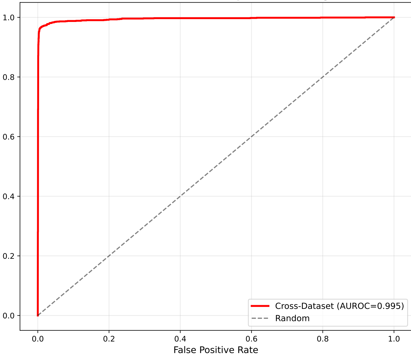
ROC Curve — Cross-Dataset (Chapman-Shaoxing → PTB-XL)
