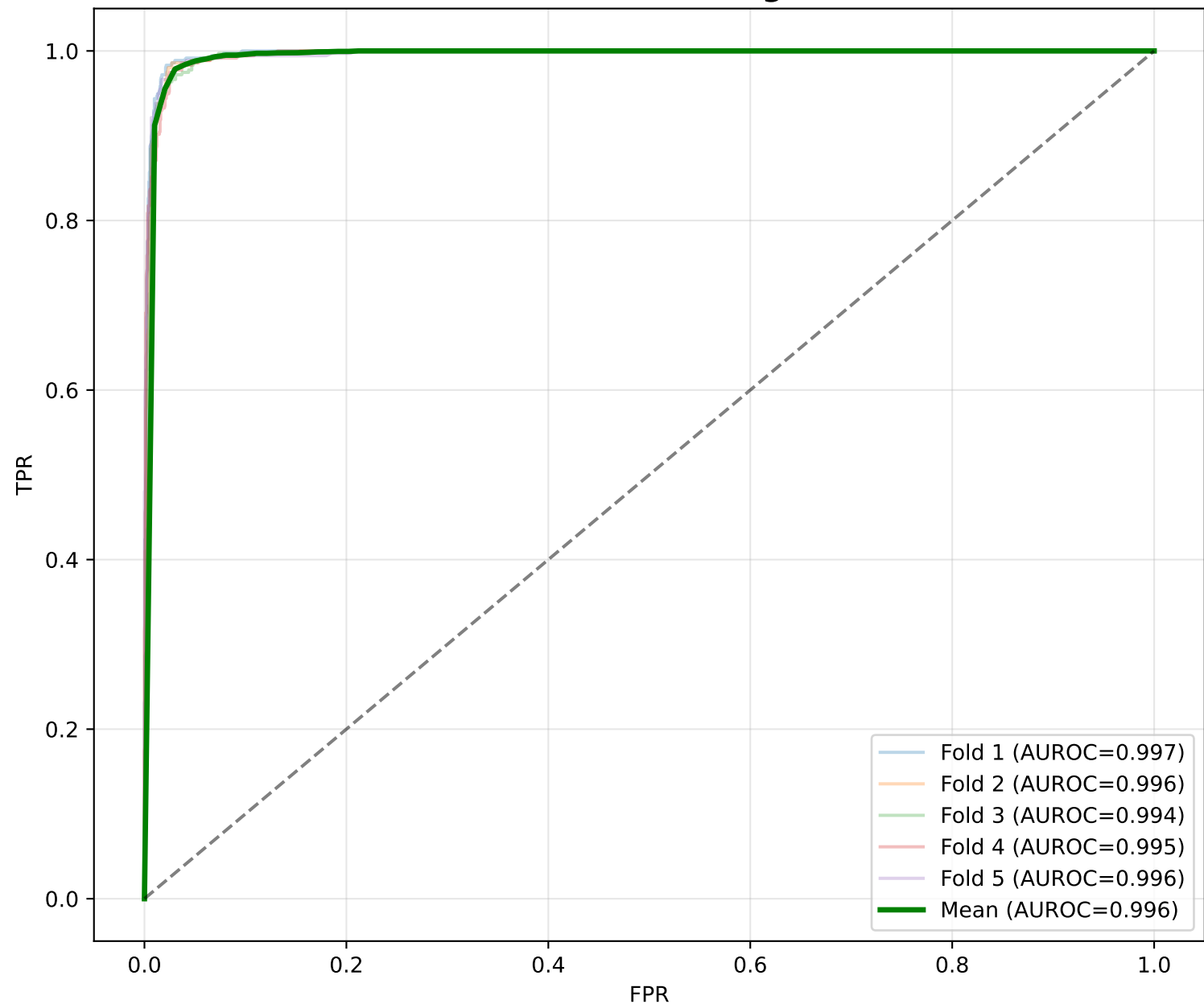
ROC — RF Full Processing All Leads
