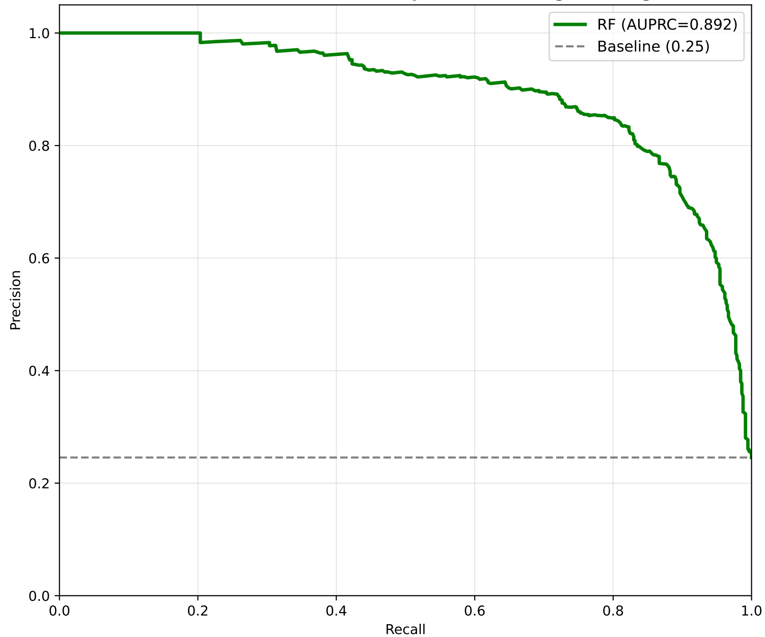
PR — RF Cross-Dataset (Chapman-Shaoxing → Georgia)
