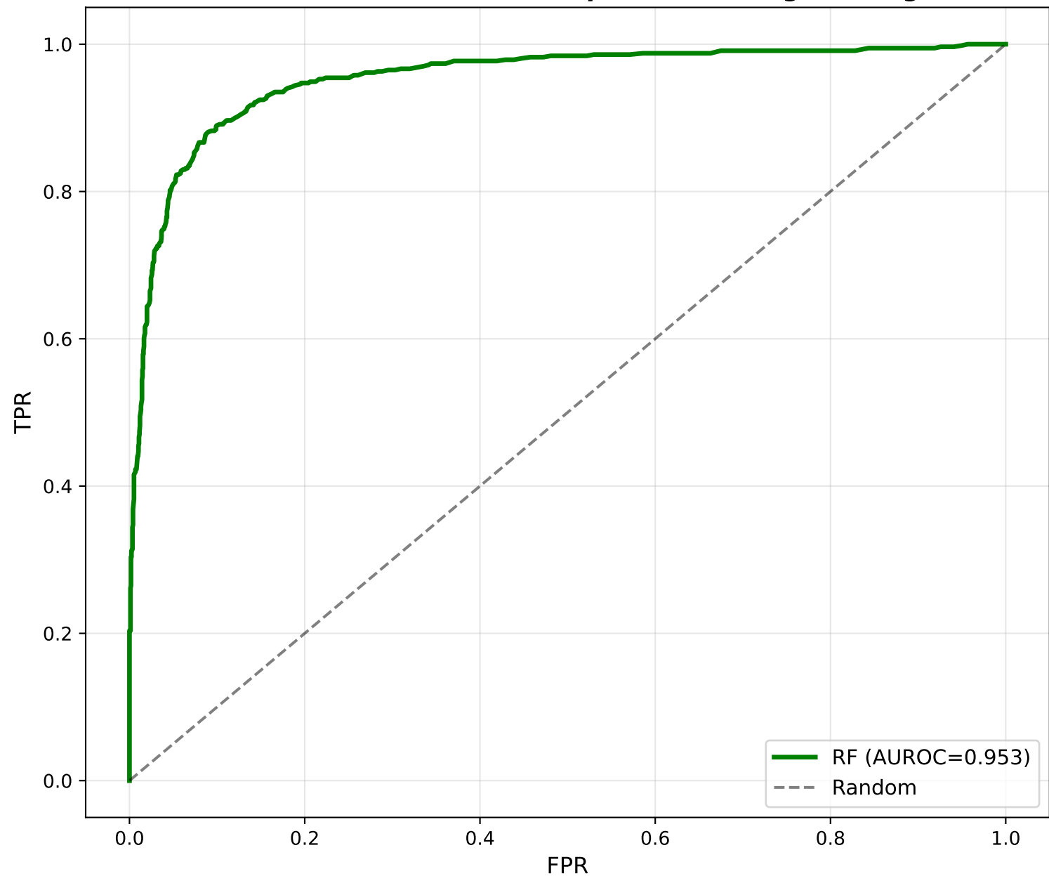
ROC — RF Cross-Dataset (Chapman-Shaoxing → Georgia)
