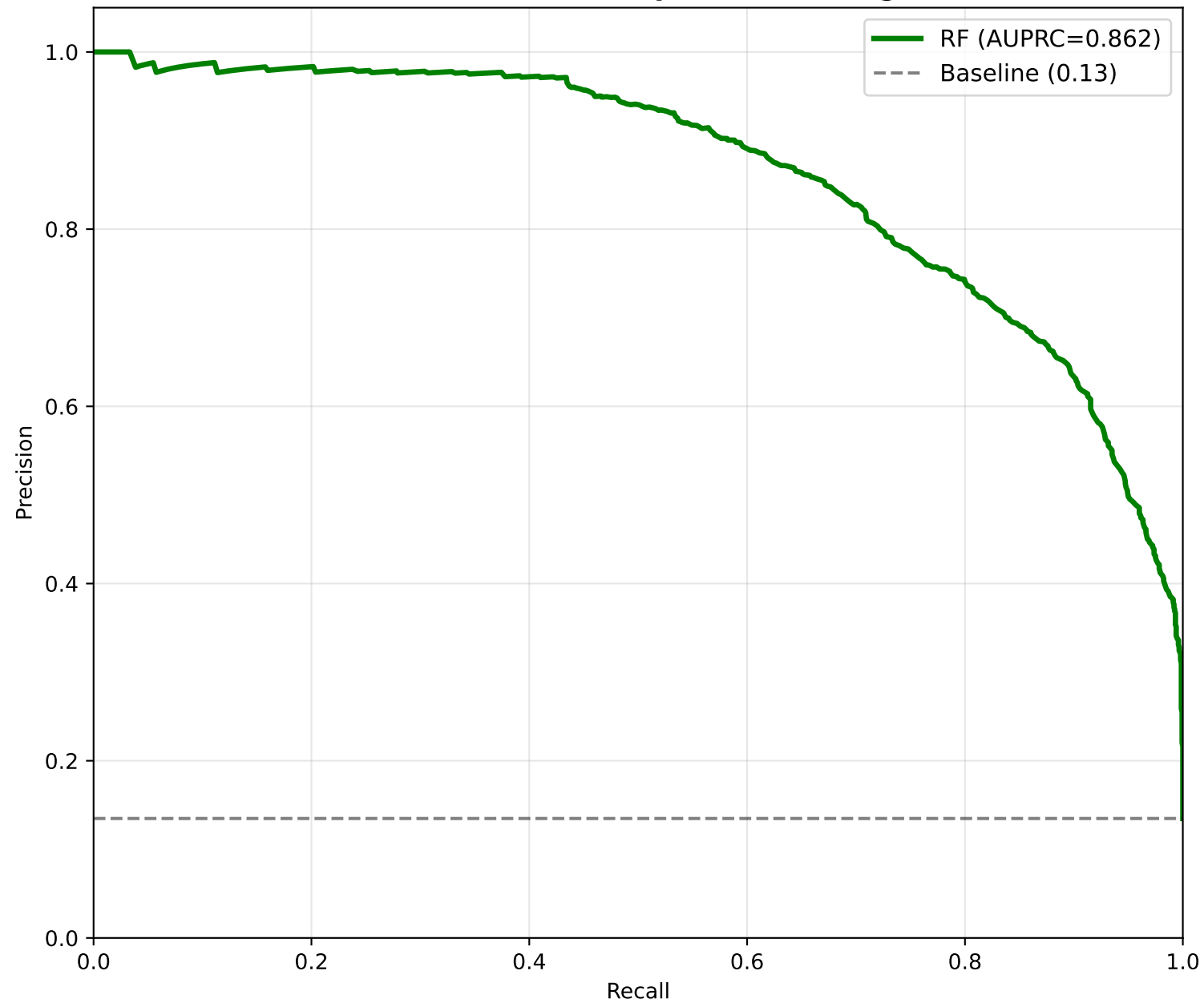
PR — RF Cross-Dataset (Chapman-Shaoxing → PTB-XL)
