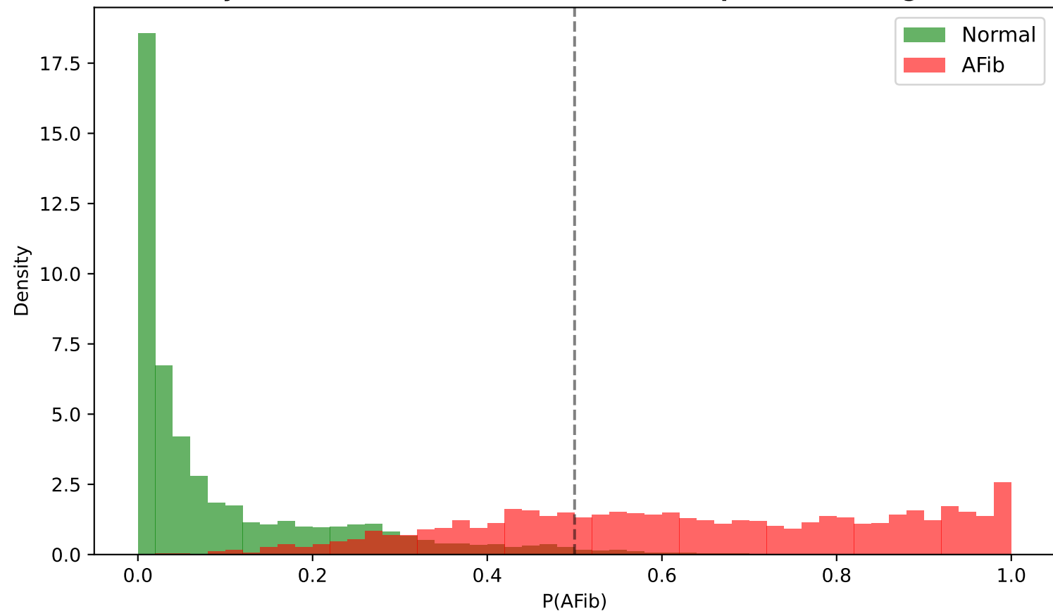
Probability Distribution — RF Cross-Dataset (Chapman-Shaoxing → PTB-XL)
