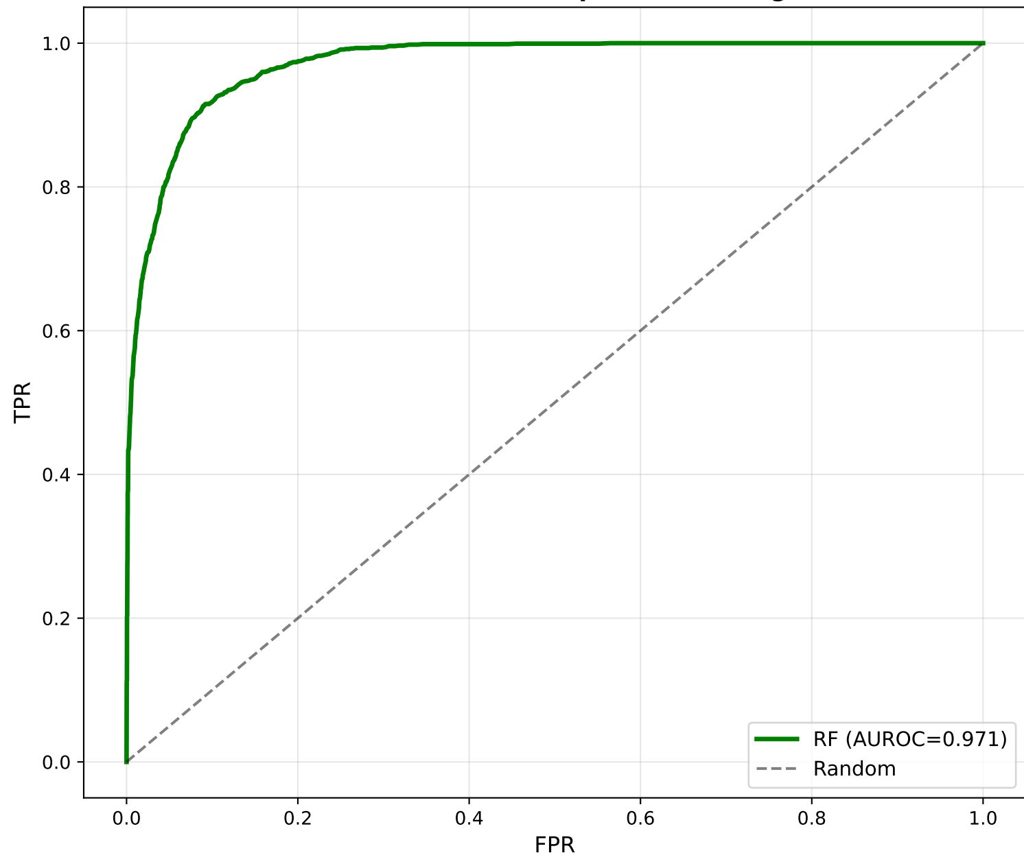
ROC — RF Cross-Dataset (Chapman-Shaoxing → PTB-XL)
