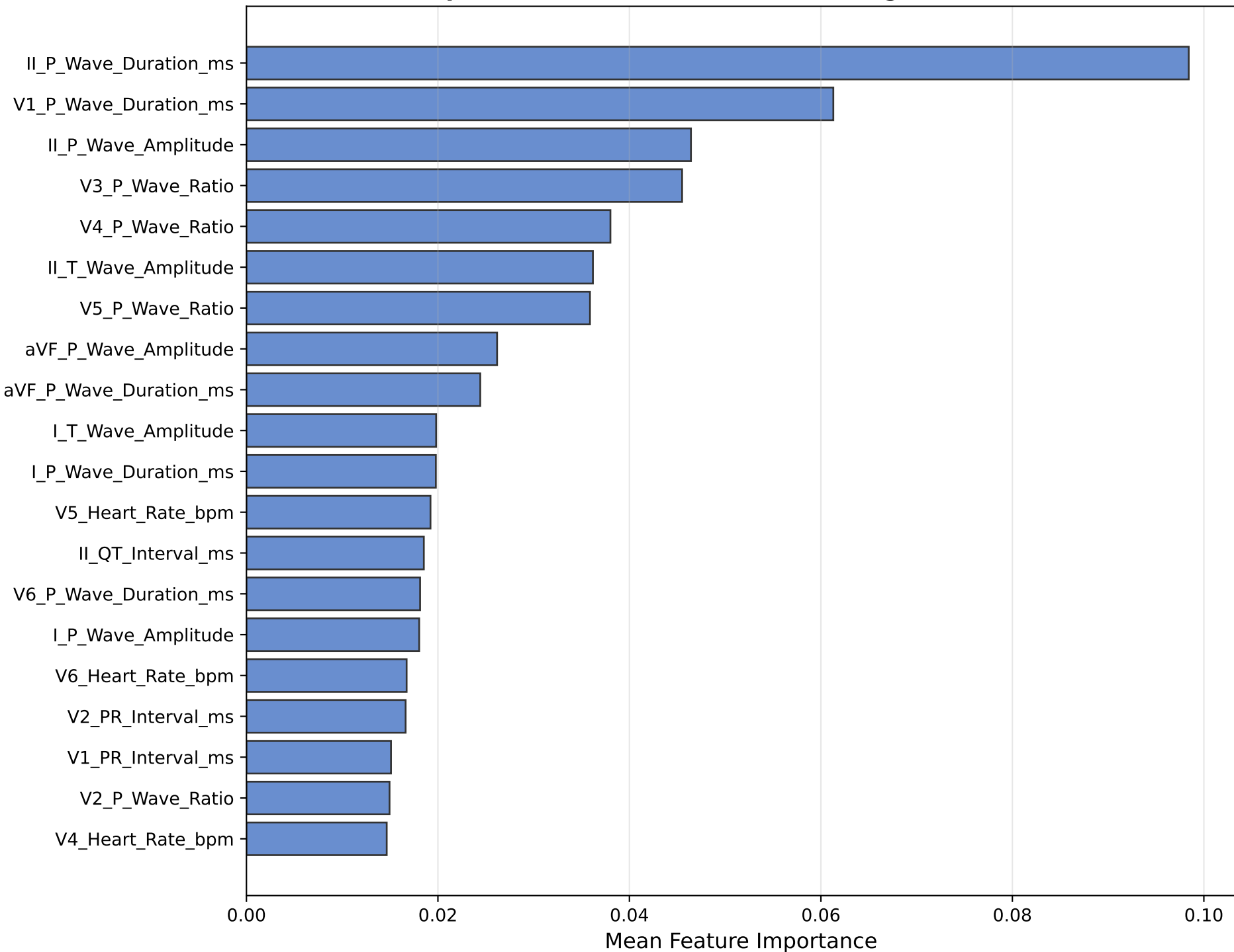
Top 20 Features — RF Full Processing All 12 Leads
