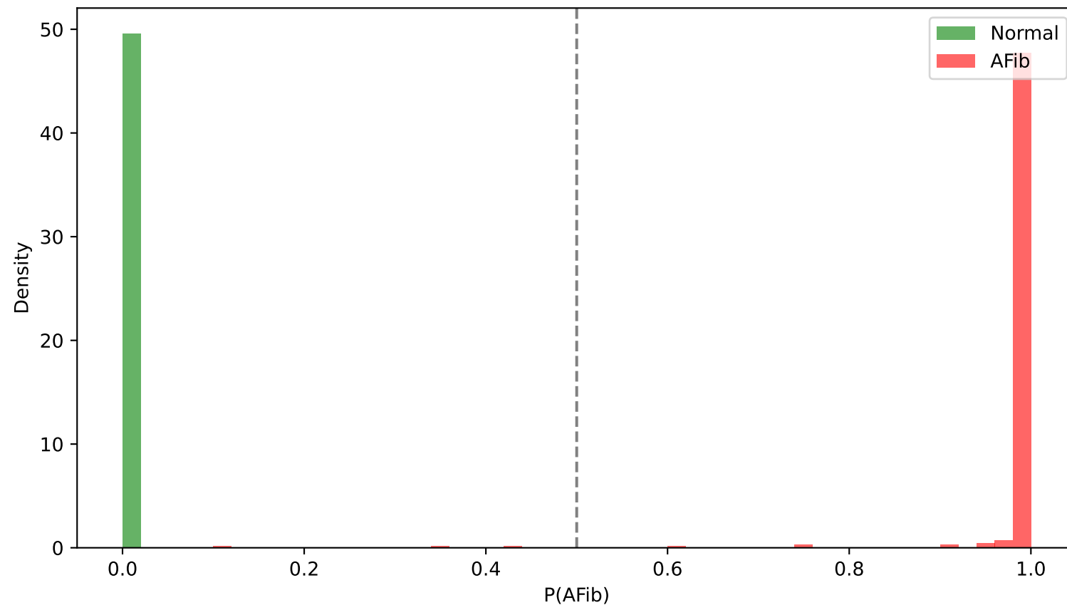
KanResWideX — After (T=1.03)
