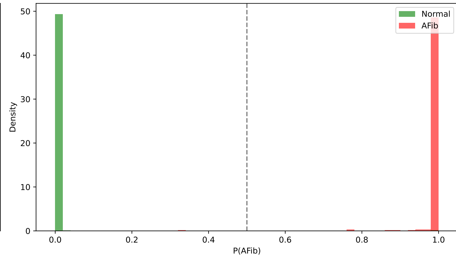
CNN-BiLSTM — After (T=1.47)
