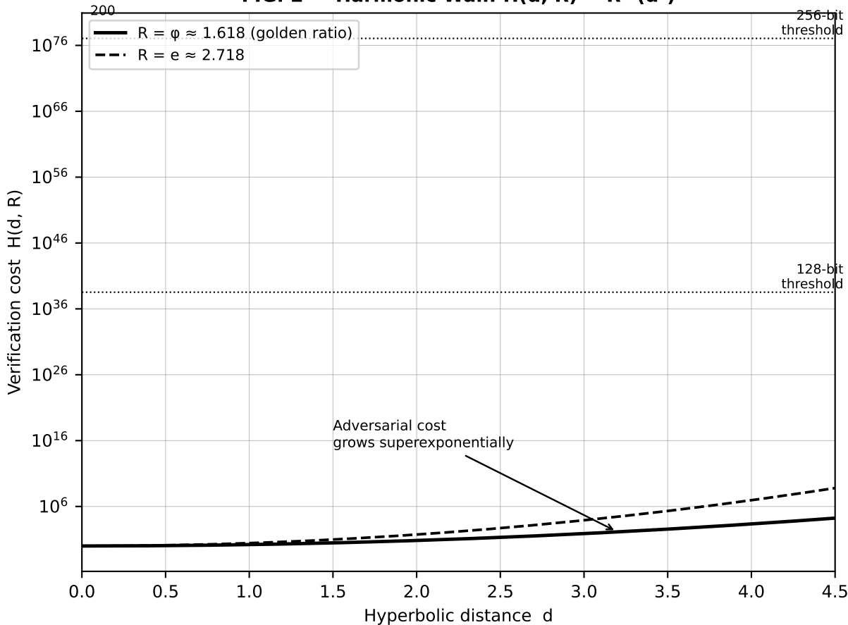
FIG. 2 — Harmonic Wall: H(d, R) = R^{(d^2)}
