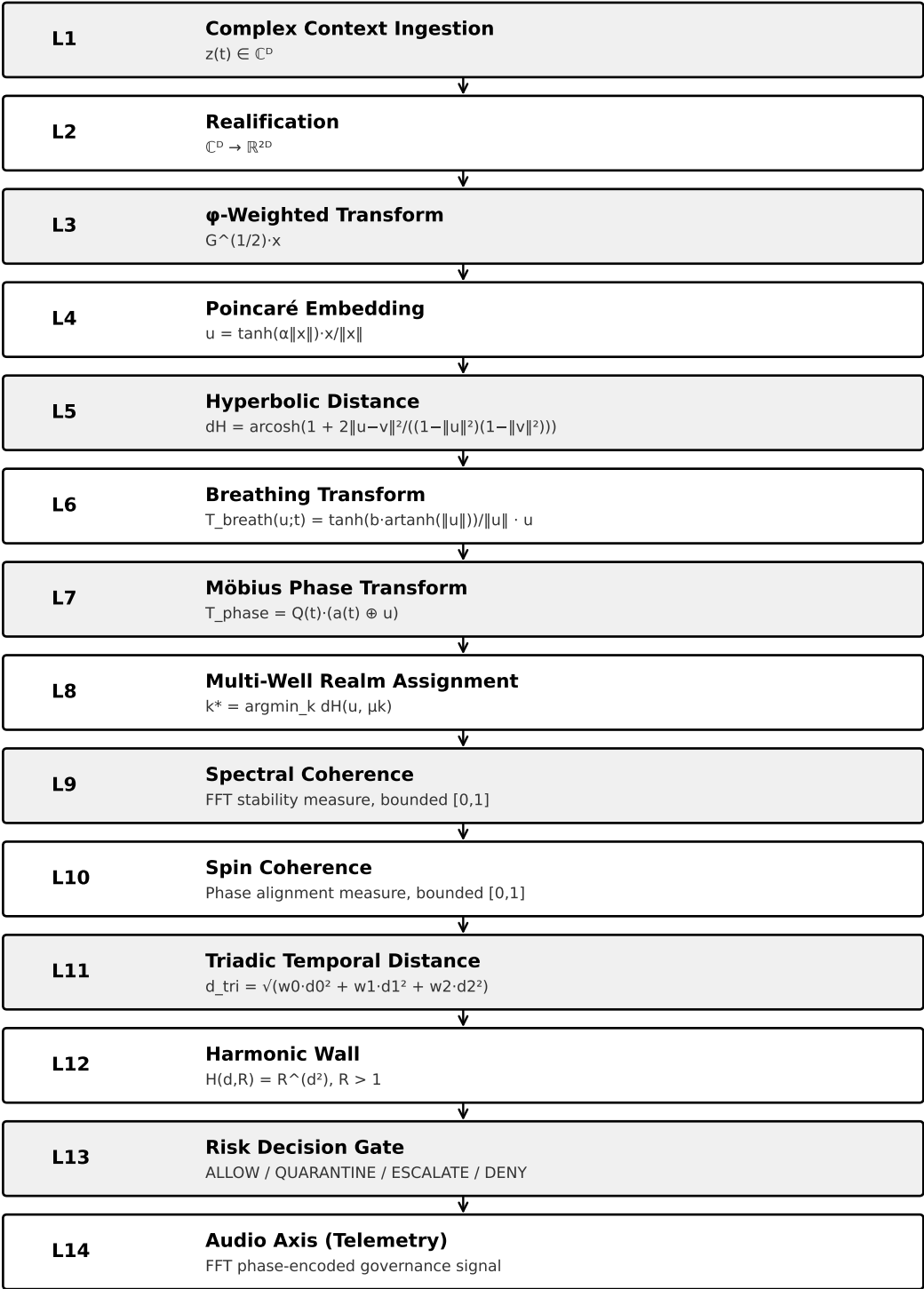
FIG. 1 14-Layer Authorization Pipeline
