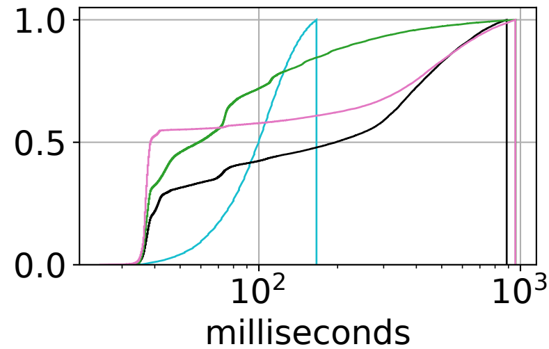
resctl
