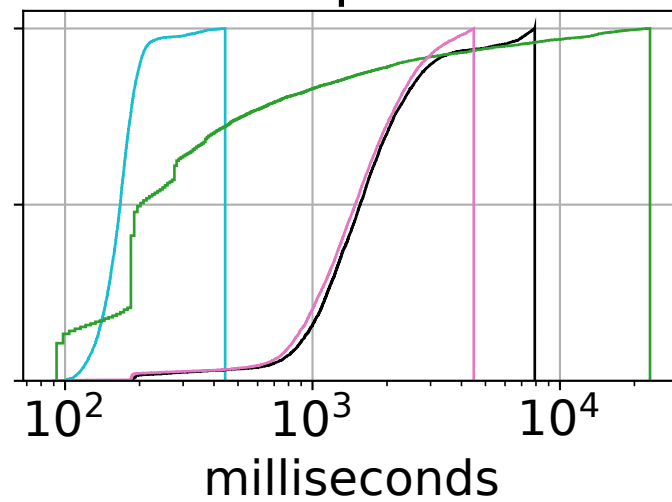
resctl-parallel
