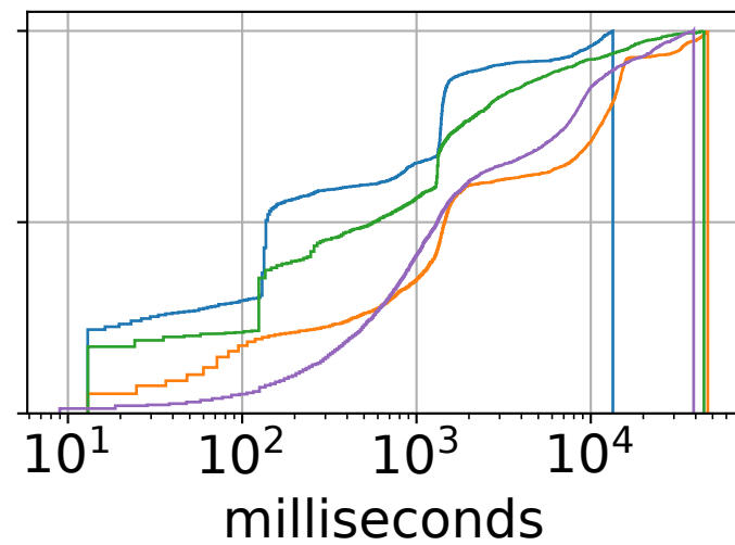
resctl-mixed
