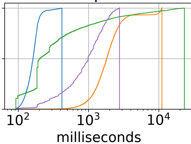
resctl-parallel
