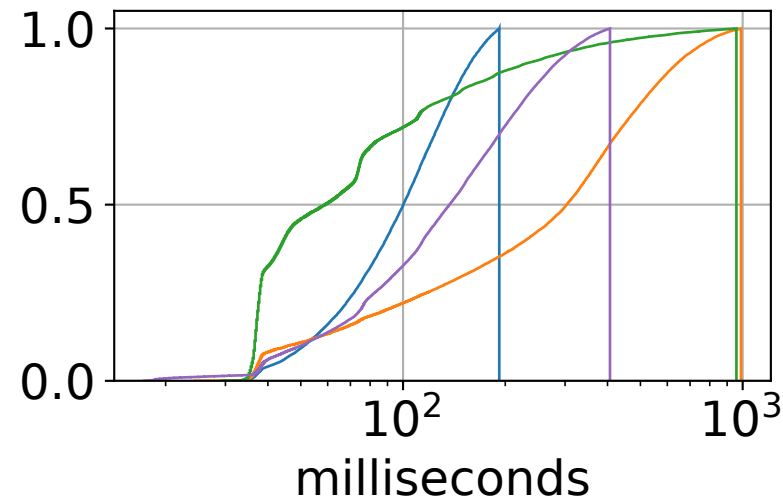
resctl
