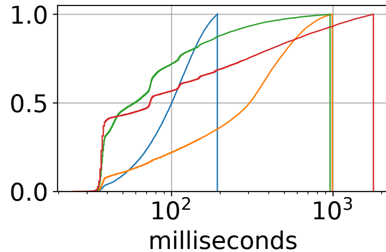
resctl
