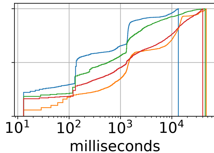
resctl-mixed
