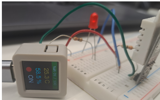
Figura 5: Circuit electric del blinking LED + DHT + Pantalla
