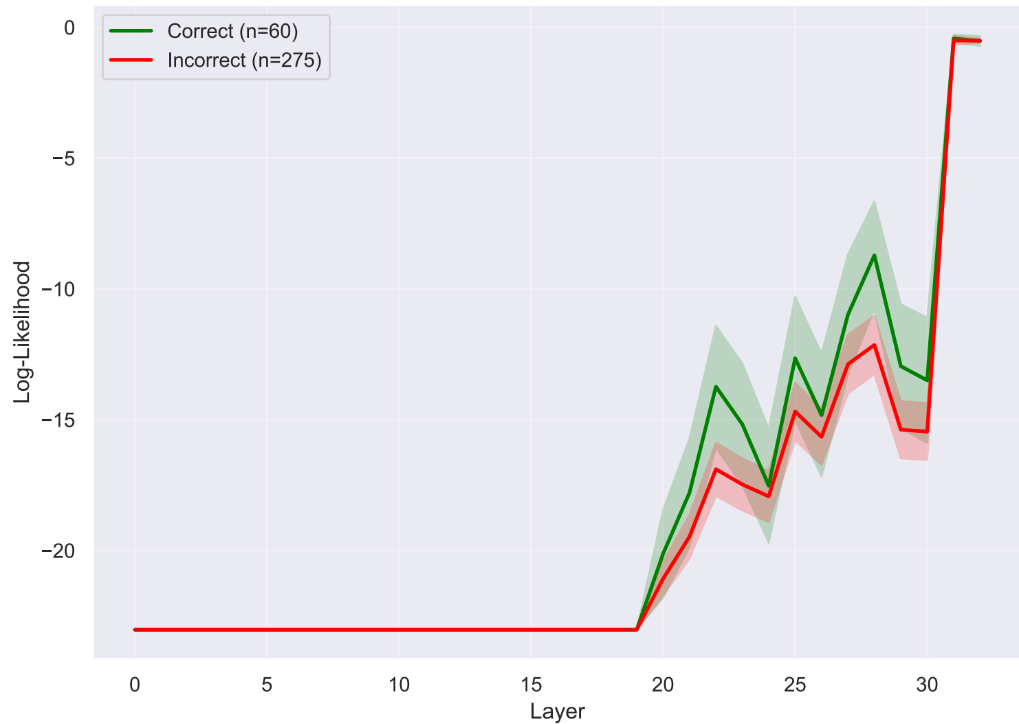
Log-Likelihood Trajectory - Bengali
