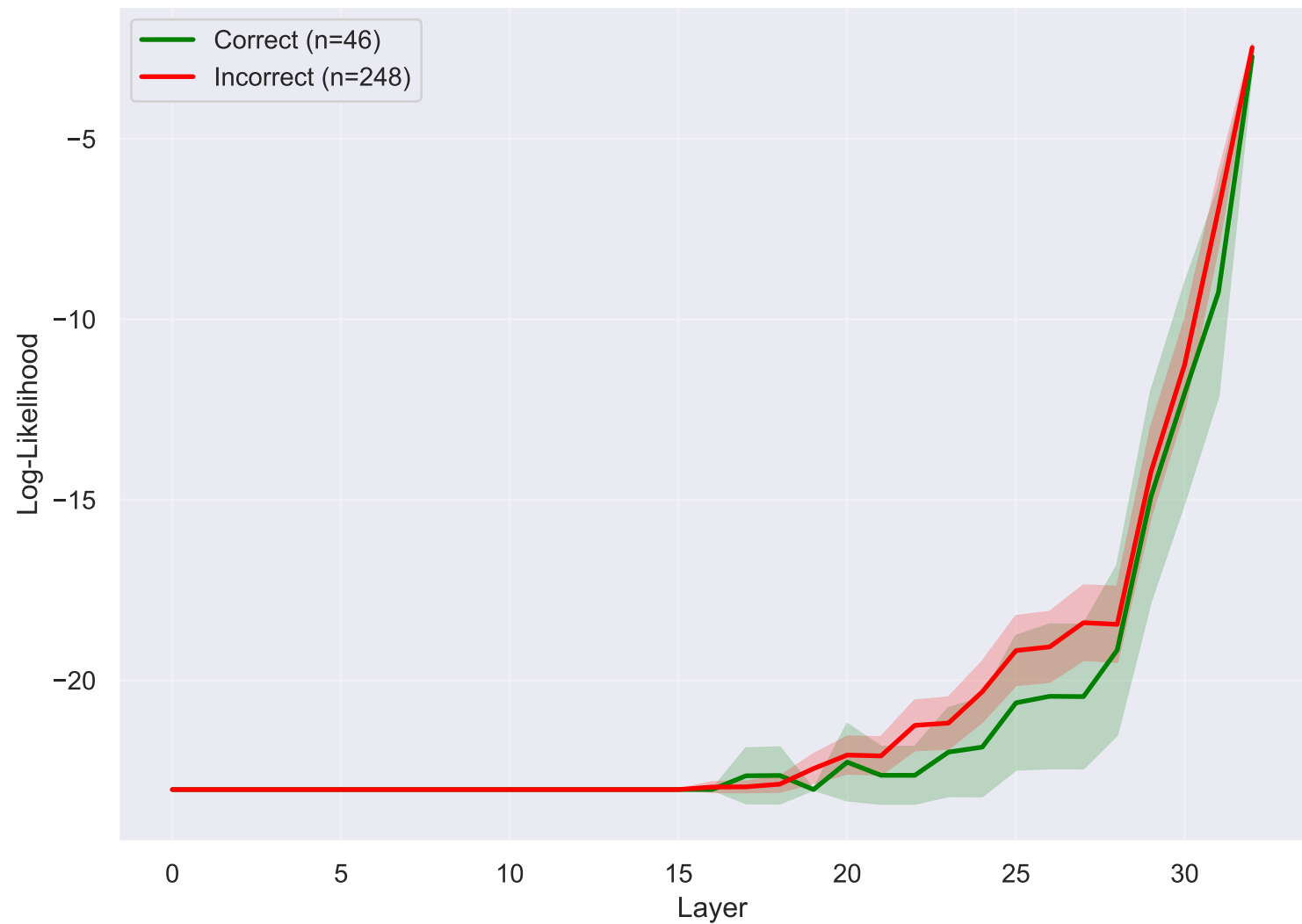
Log-Likelihood Trajectory - Spanish
