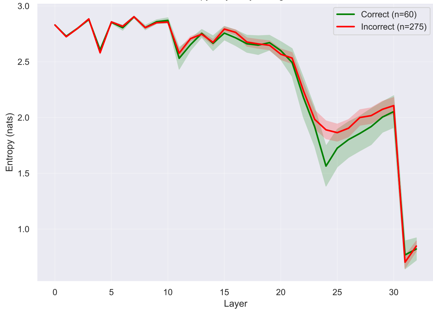
Entropy Trajectory - Bengali
