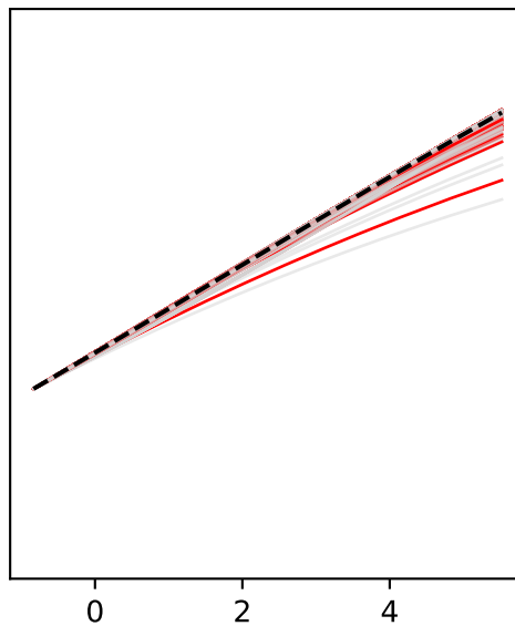
characteristic_distance
