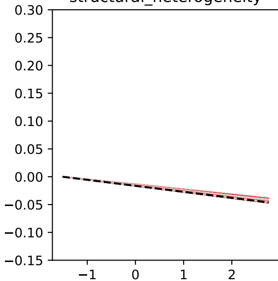
structural_heterogeneity
