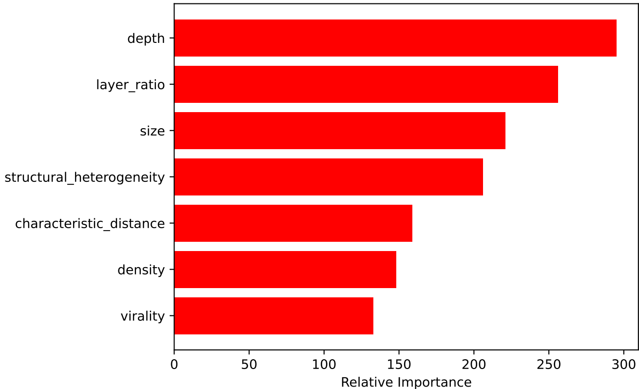
Feature Importances
