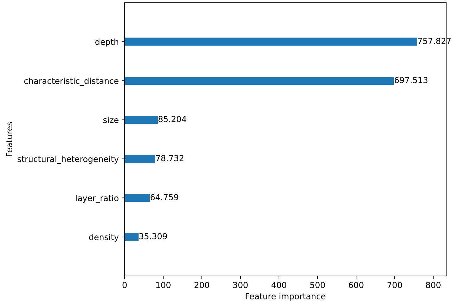
LightGBM Feature Importance (Gain)
