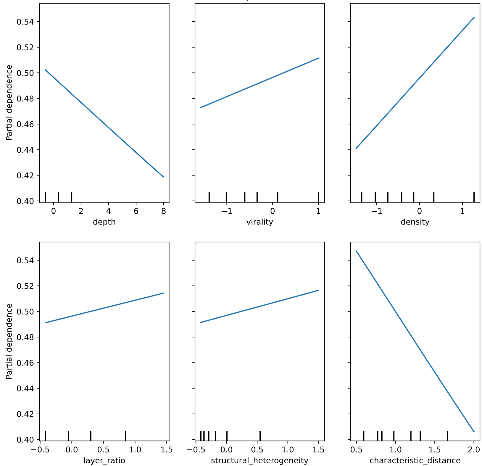
Partial Dependence Plots
