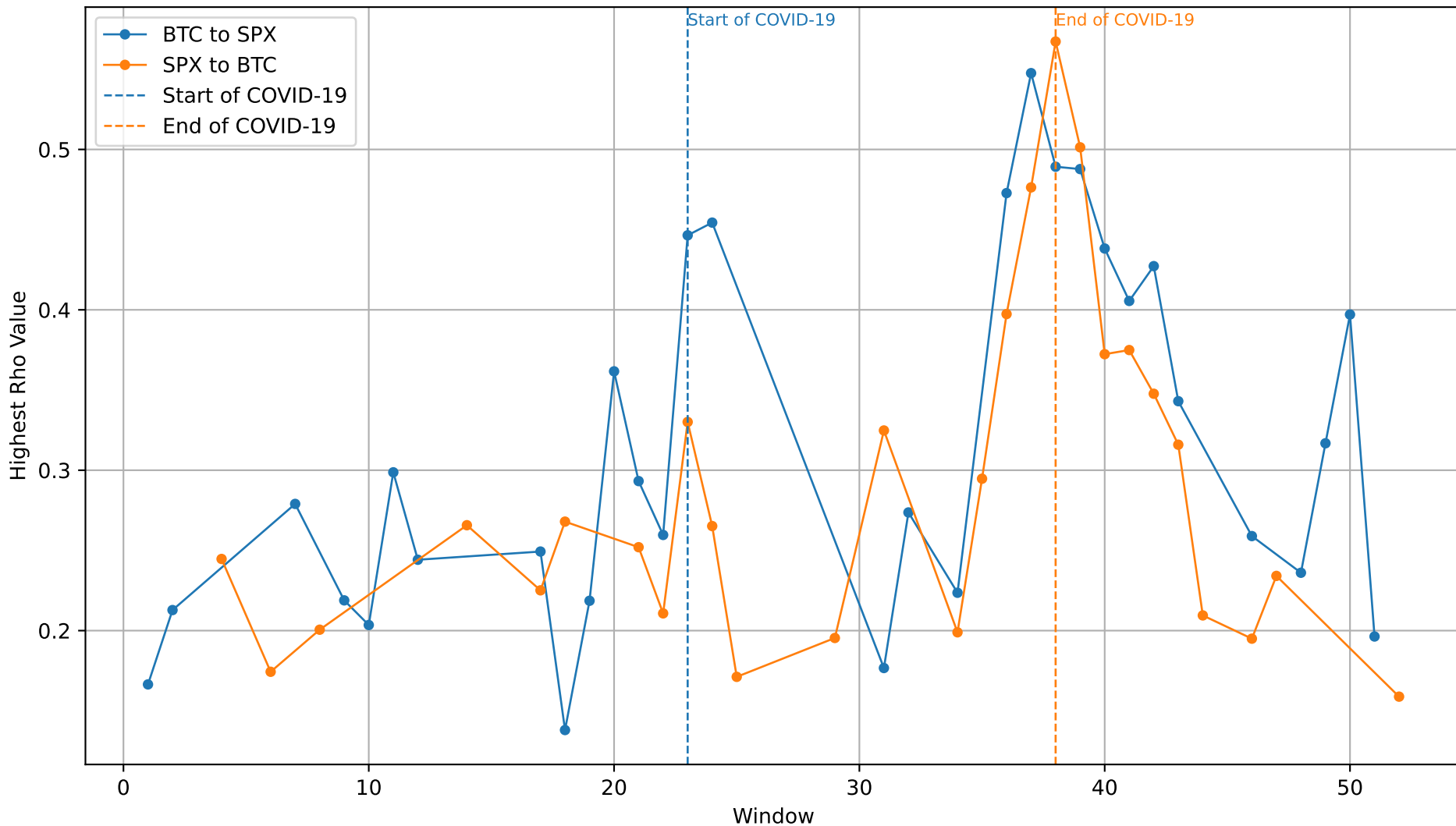
Highest Rho Value per Window for BTC and SPX (log returns)
