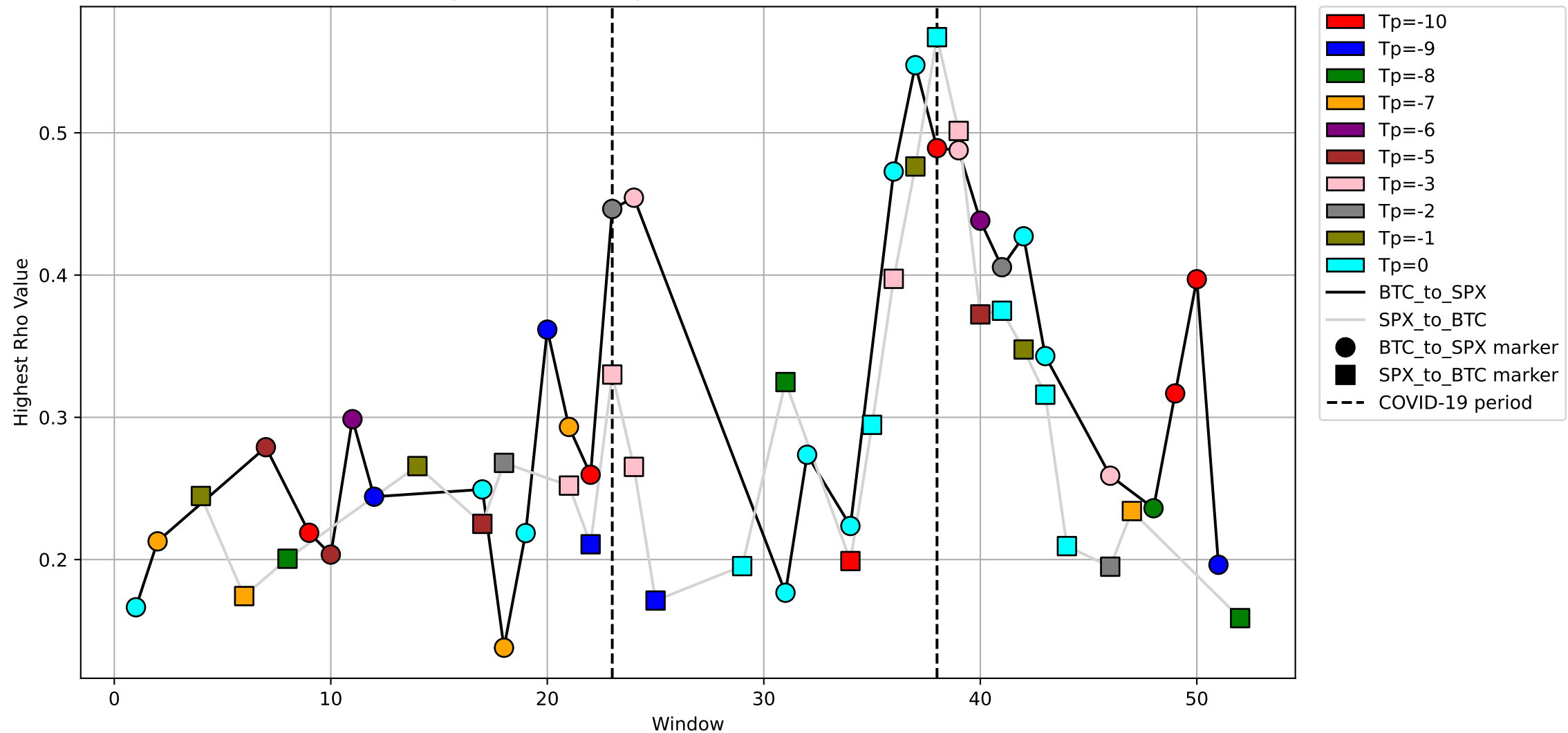
Highest Rho Value per Window for BTC and SPX
