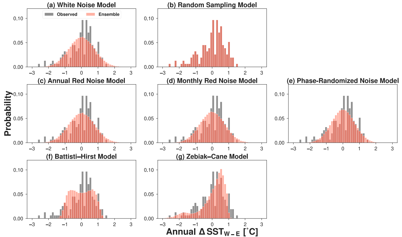
FIG. 3. The observed distribution (gray) of annual \Delta\text{SST}_{\text{W-E}} values, compared with the ensemble distribution of (a) annual Gaussian white noise time series, (b) annual time series with randomly sampled observed annual \Delta\text{SST}_{\text{W-E}} values, (c) annual red noise time series constructed using the observed annual AR1 coefficient, (d) monthly red noise time series constructed using the observed month-specific AR1 coefficients, (e) monthly time series with randomly shifted phases, (f) monthly time series constructed using the Battisti and Hirst (1989) conceptual model, and (g) monthly time series randomly sampled from a 100 000-yr unforced simulation of the Zebiak–Cane model. The ensemble distributions of all statistical and physical models are shown in red.
