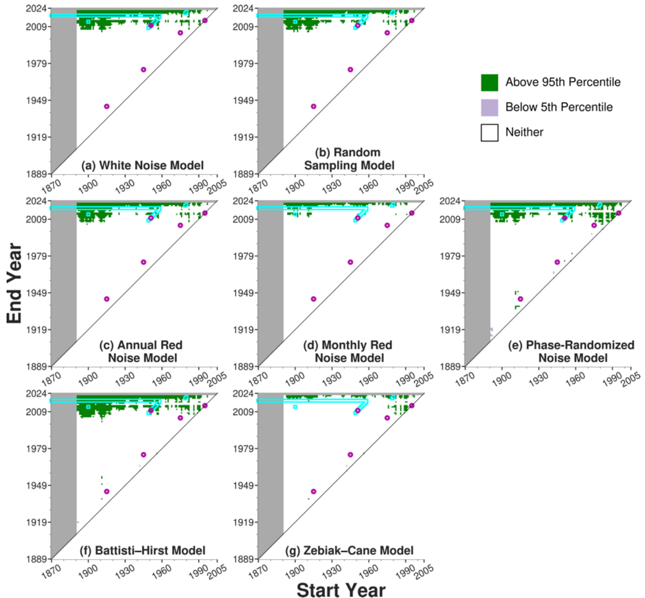
FIG. 8. As in Fig. 6, but using COBE data. The gray shading notes COBE's reduced temporal coverage relative to the other datasets.
