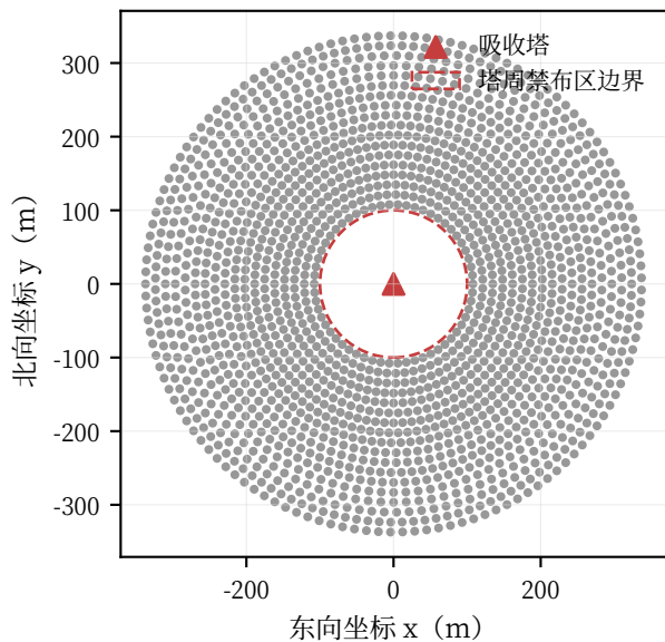
(a) 镜场平面布置 (1745面)
