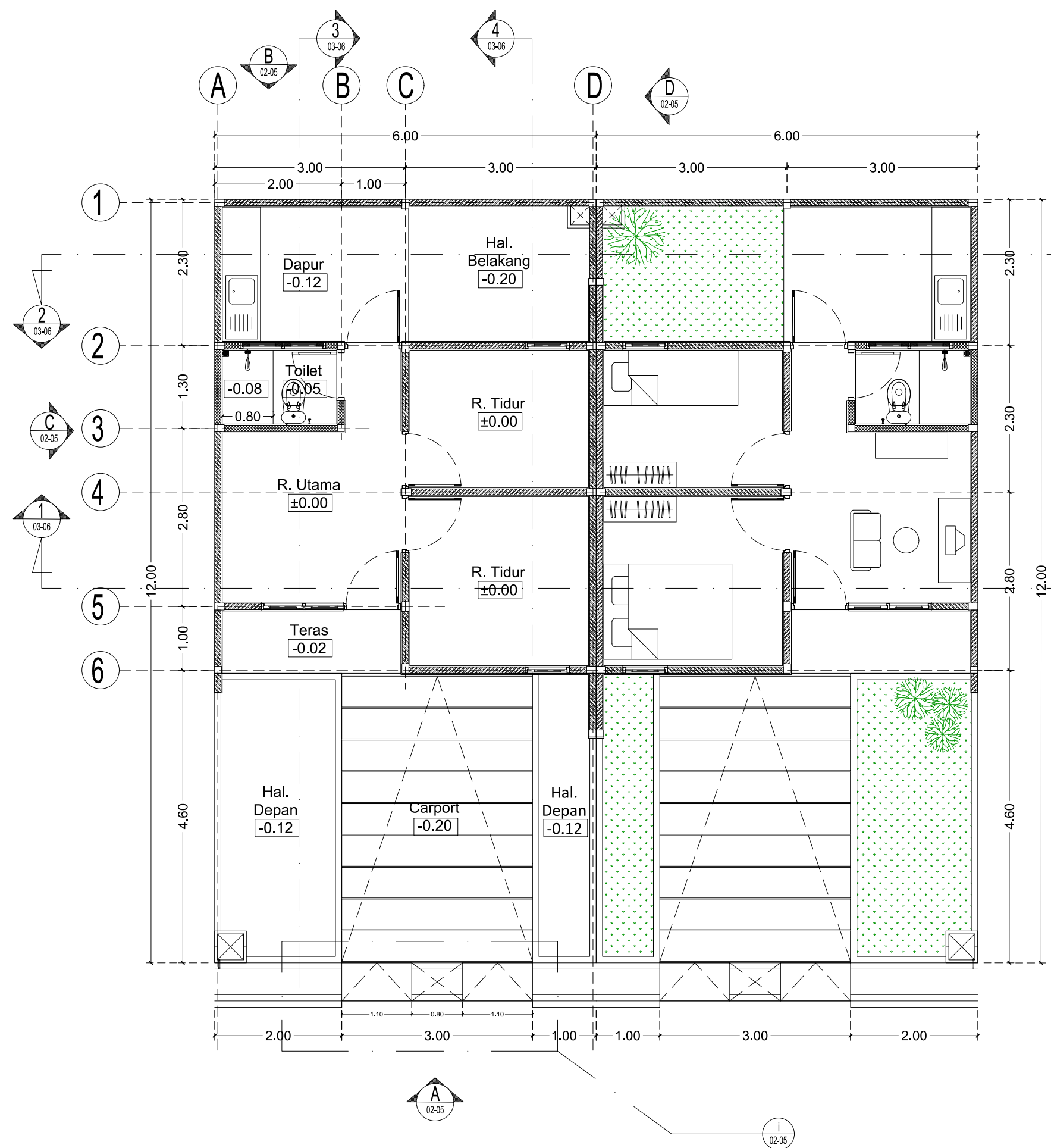
A Denah A-01-04 Skala 1:100
