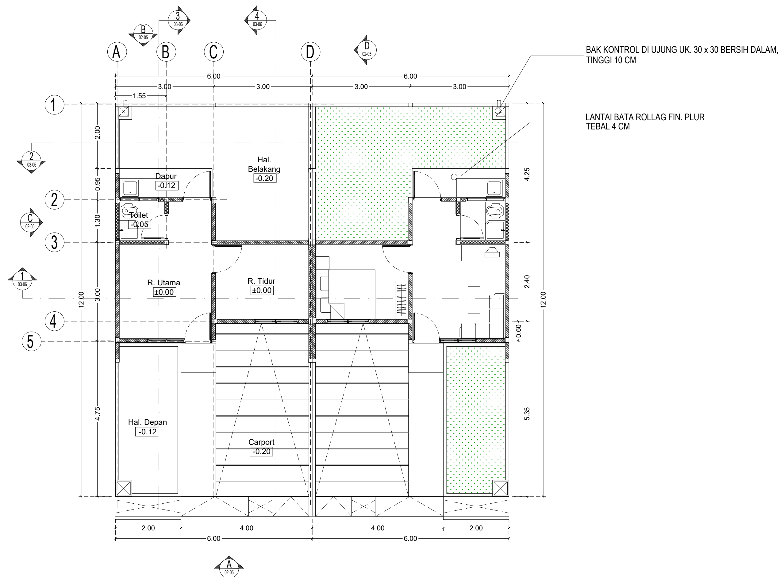
A Denah A-01-04 Skala 1:100
