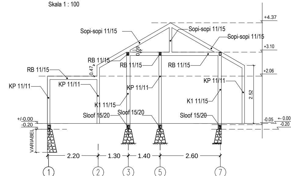
PORTAL As D Skala 1 : 100
