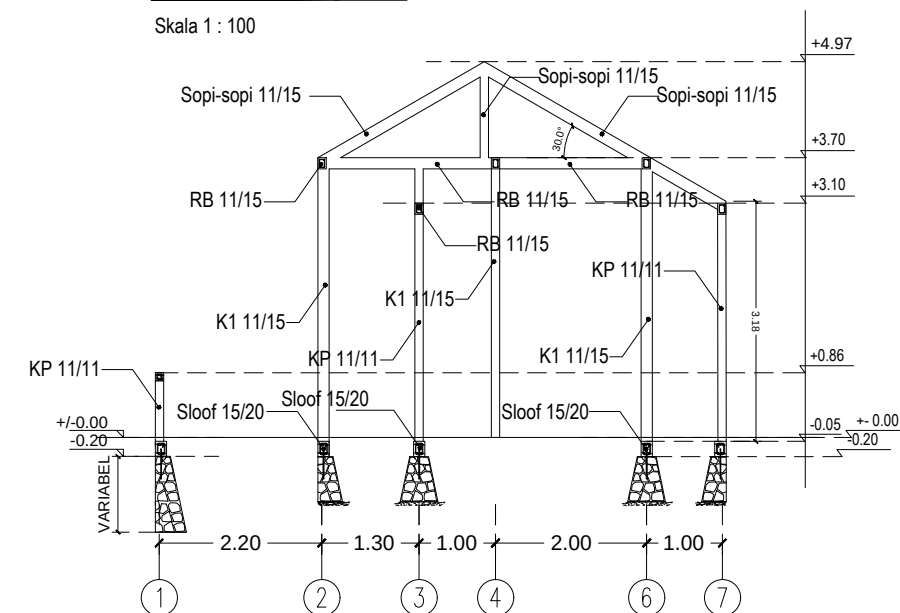
PORTAL As B Skala 1 : 100
