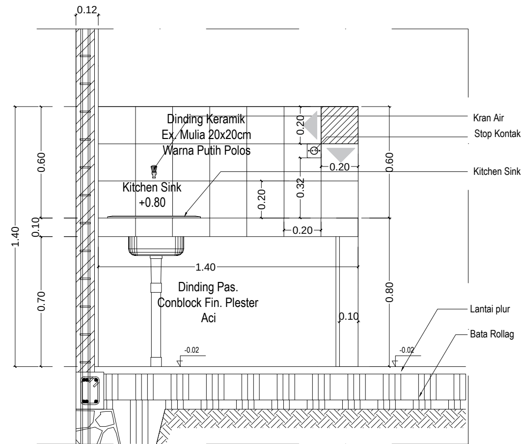
DETAIL Dapur I
