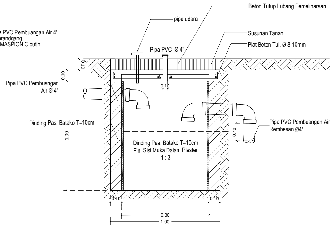
DETAIL Septictank
