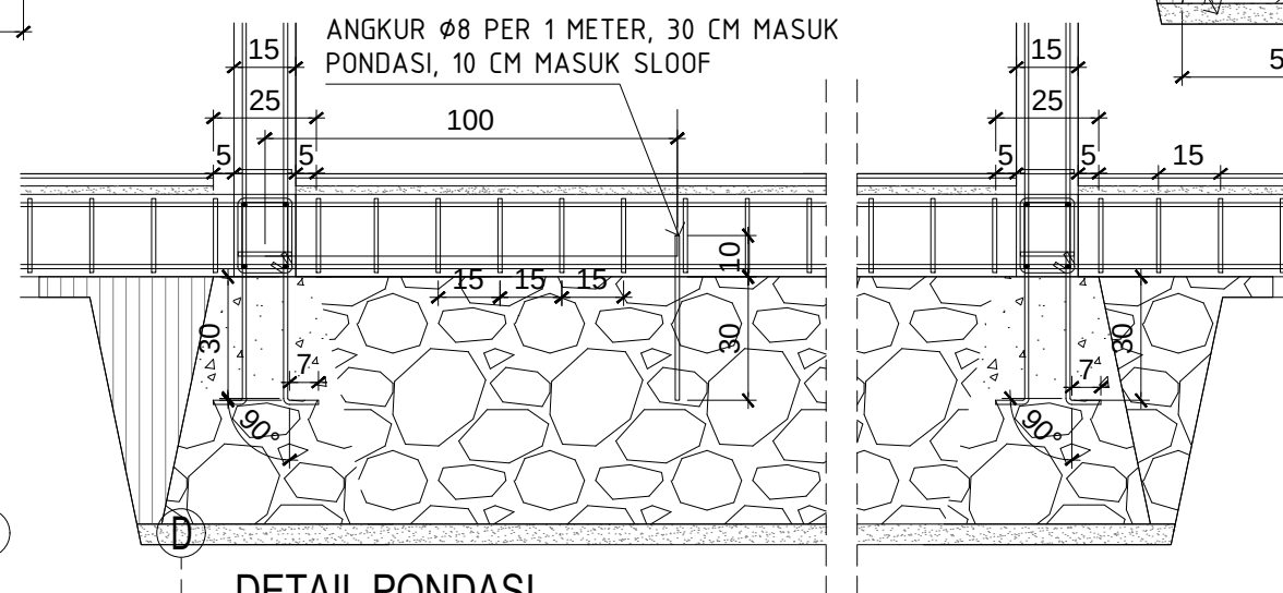
DETAIL PONDASI Skala 1:50
