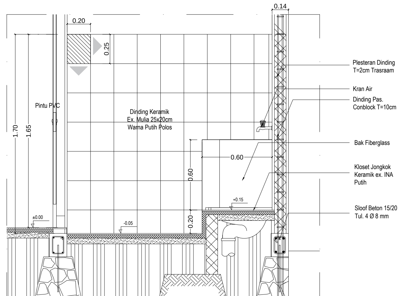
DETAIL Toilet II
