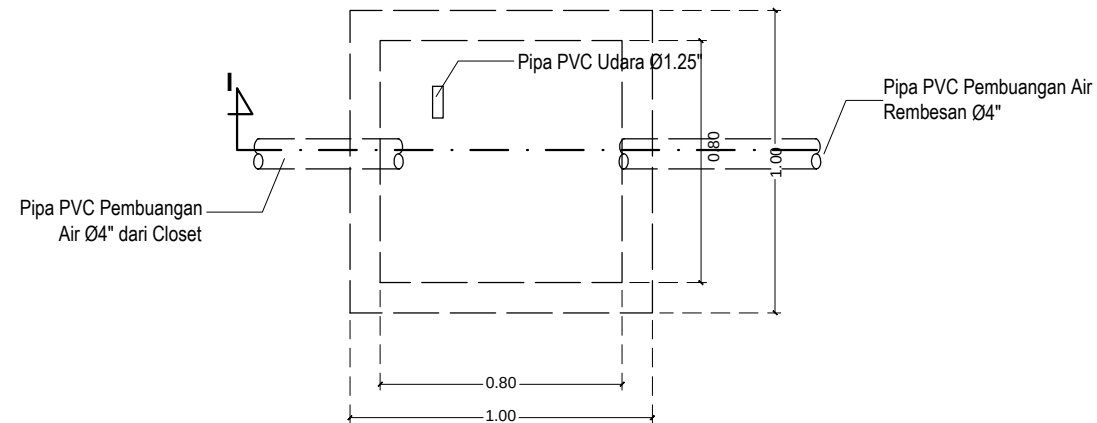
Denah Septictank
