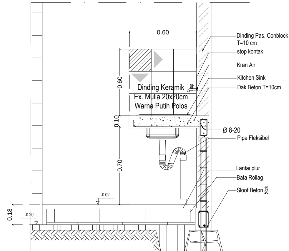
DETAIL Dapur II
