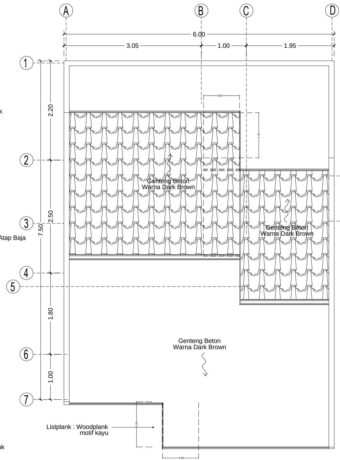
DENAH ATAP
