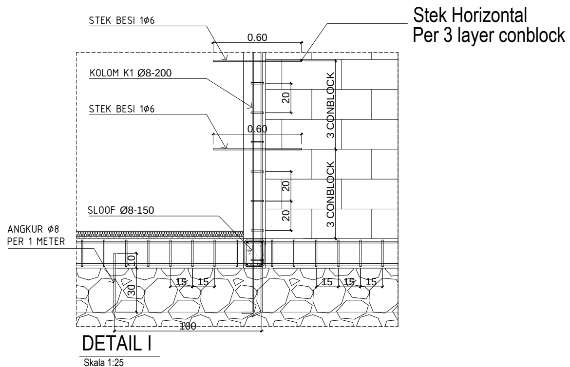
DETAIL I
