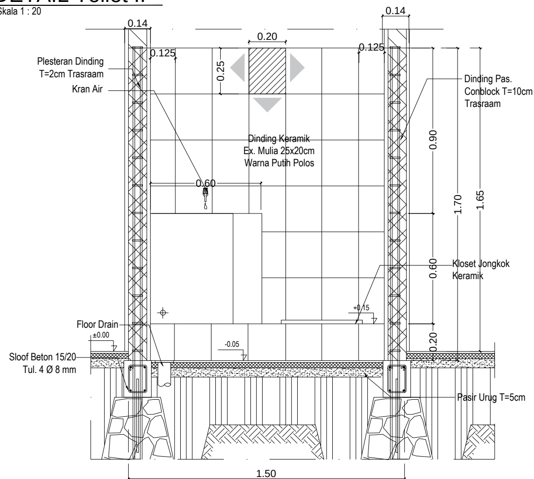
DETAIL Toilet I
