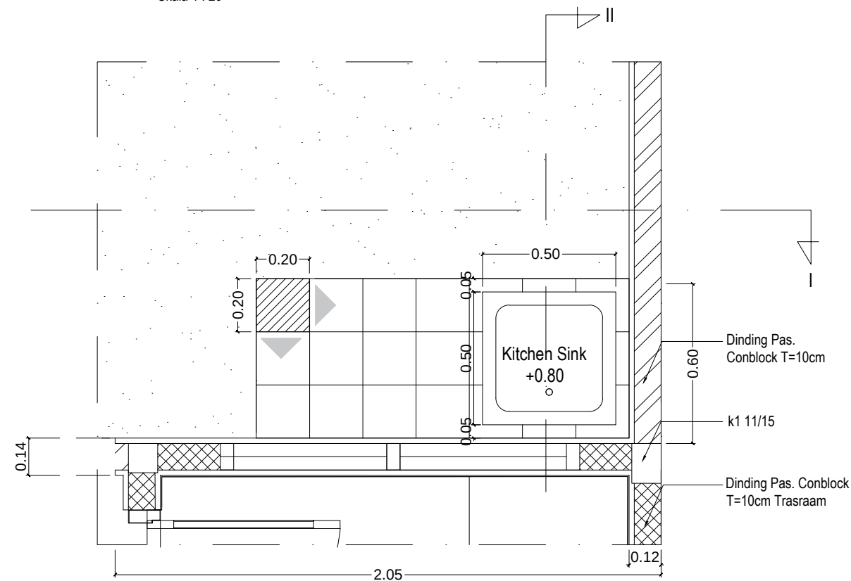
Denah Dapur
