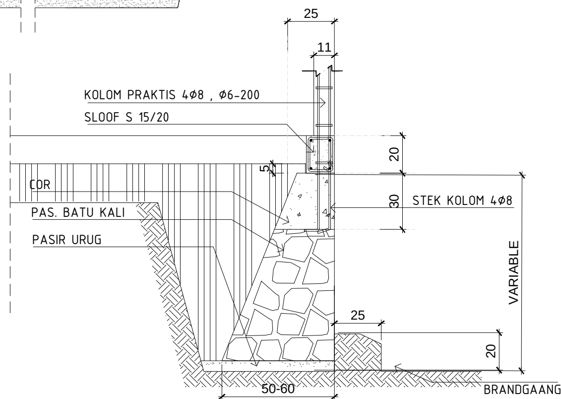
DETAIL PONDASI P3 Skala 1:50
