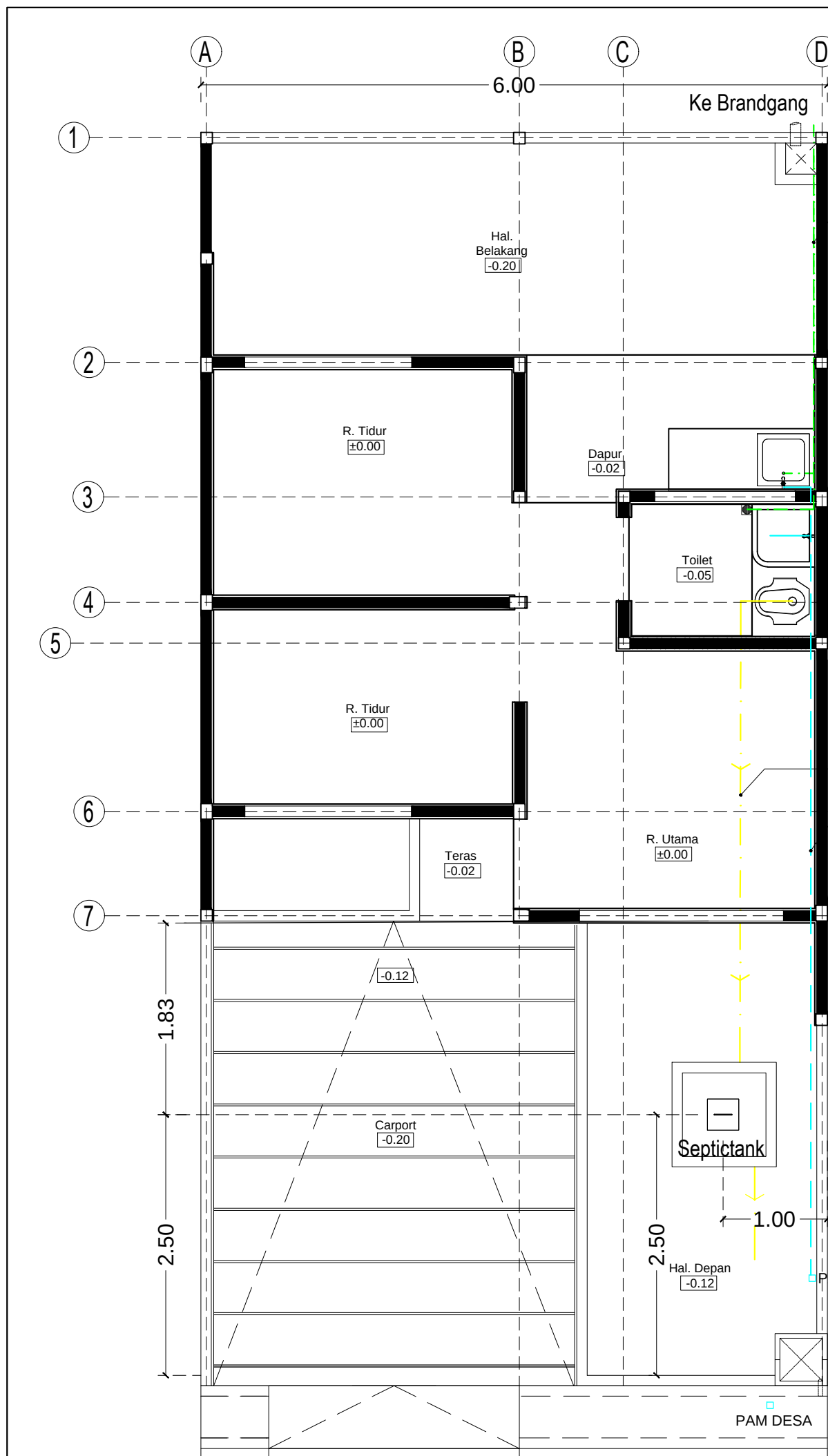
Denah Instalasi Air
