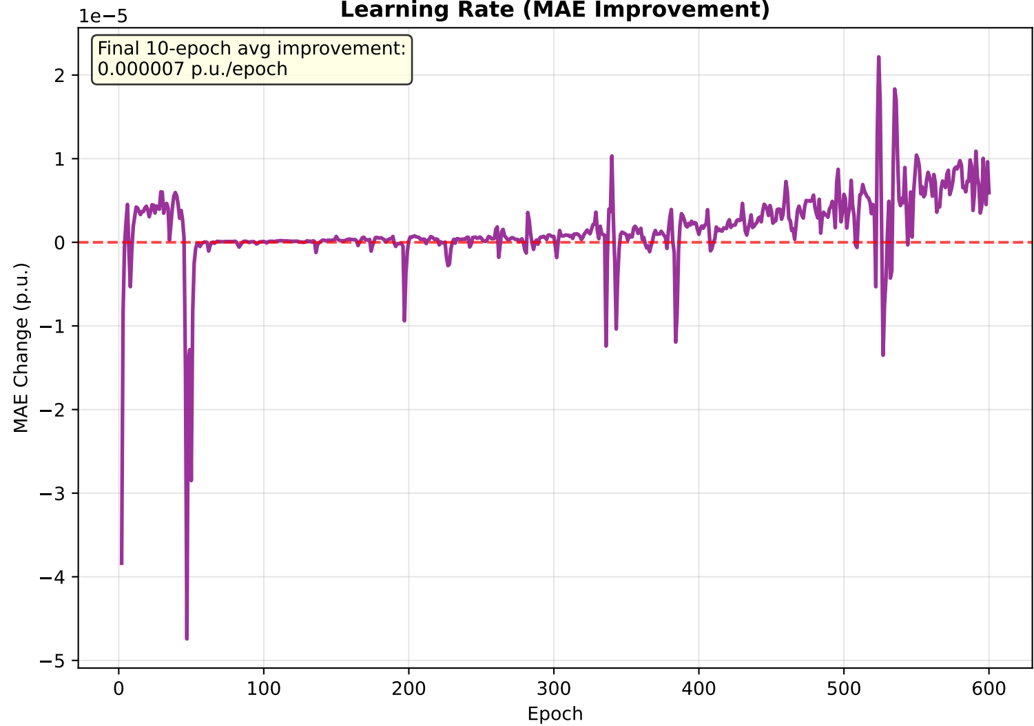
Learning Rate (MAE Improvement)
