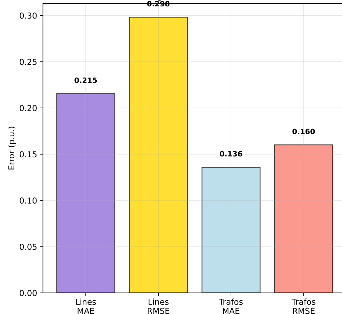
Loading Estimation Metrics
