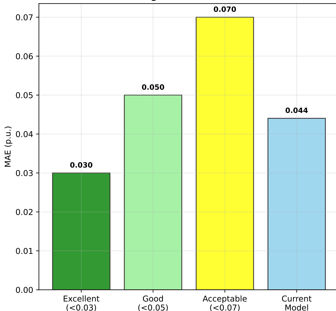
Voltage MAE Benchmark
