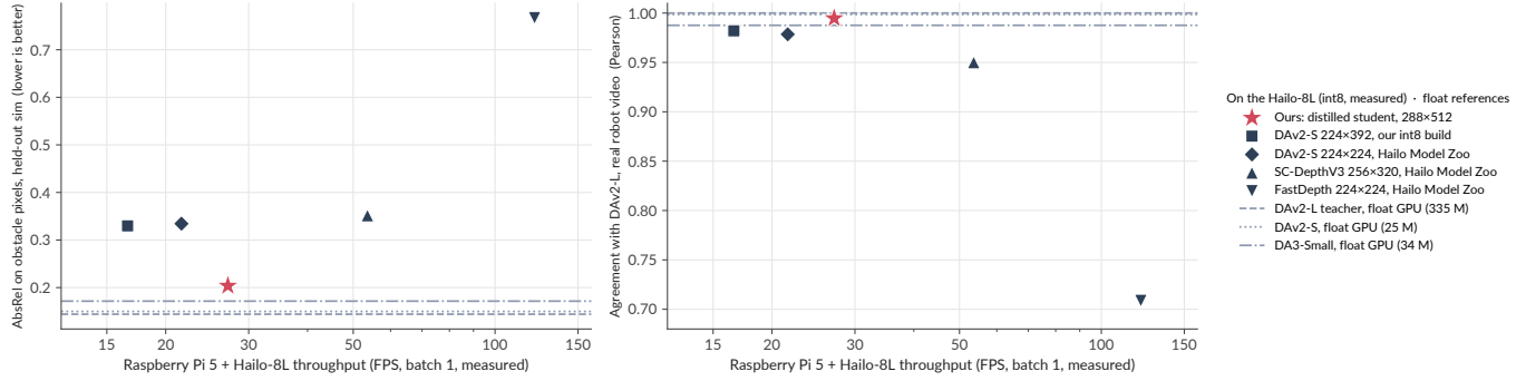
Fig. 4. Accuracy against measured on-chip throughput on the Raspberry Pi 5 + Hailo-8L (batch 1). Left: AbsRel on obstacle pixels. Right: agreement with Depth Anything V2-Large on real robot video. Horizontal lines: float GPU models that cannot run on the Pi at this rate.
