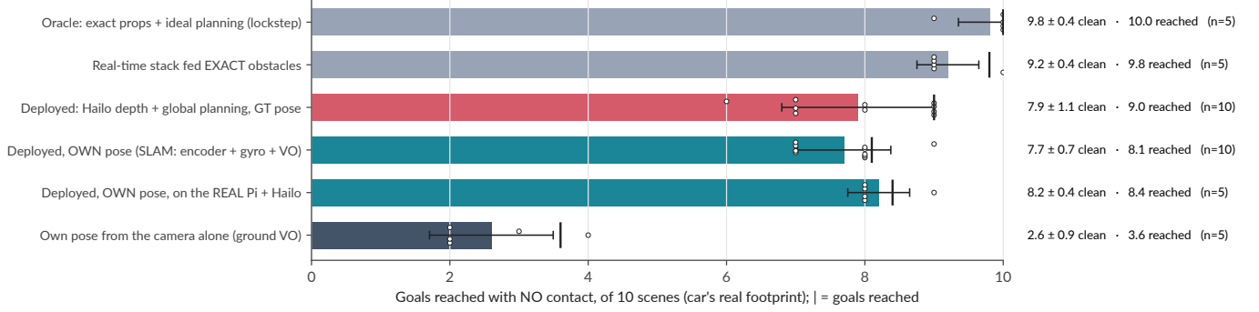
Hardware-in-the-loop yard suite, real time: what perception and self-localisation cost
