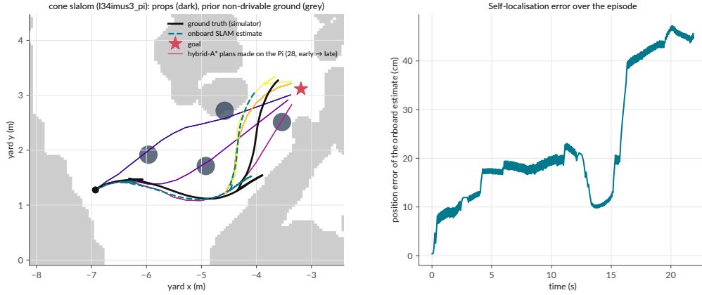
Fig. 7. Onboard SLAM and global planning on the robot’s own pose: every hybrid-A* plan the Pi made in one cone-slalom episode, the SLAM estimate against the truth, and the localisation error over time. The car reached the goal despite 0.47 m peak drift.
