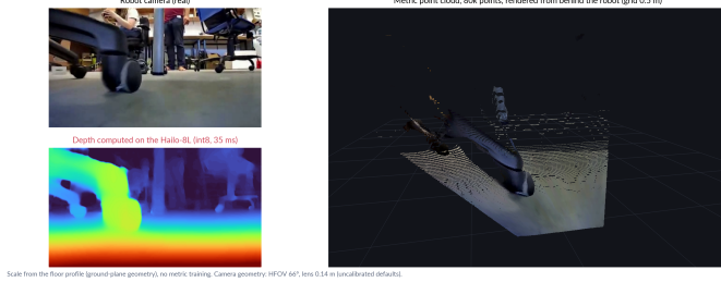
Fig. 5. A real robot frame lifted to metric 3D on the Pi: chip depth, scale from the floor profile, flying pixels removed.
