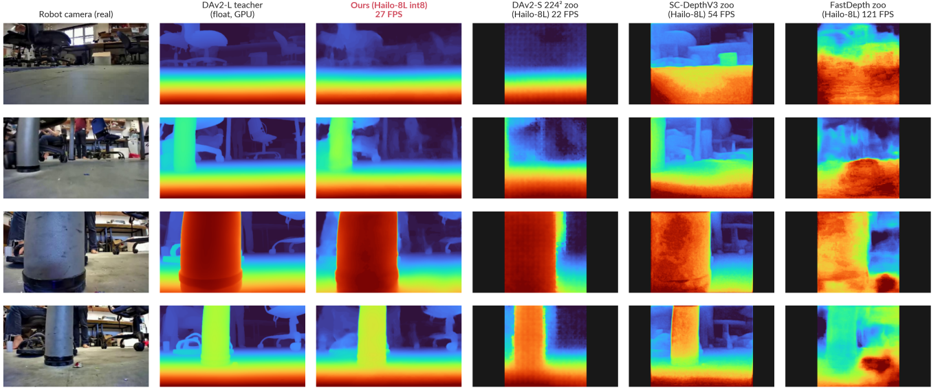
Fig. 1. Depth computed on the Hailo-8L for real robot frames, against the float Depth Anything V2-Large teacher on a GPU. Our attention-free student keeps the teacher’s structure at 27 FPS; the int8 transformer builds (ours and Hailo’s Model Zoo) lose it, and the small self-supervised zoo models are coarse. Dark areas lie outside a model’s input crop.
