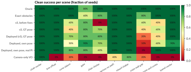
Fig. 10. Clean success per scene (fraction of seeds). Failures concentrate on the cone slalom, the gate, the chair cluster, the crate wall and the person-and-cones scene.
