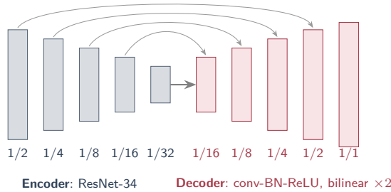
no attention, LayerNorm or softmax; 24.5 M parameters; 35.1 ms on the Hailo-8L
