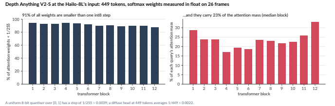
Fig. 2. Float Depth Anything V2-Small at the Hailo-8L’s 449-token input: per block, the share of softmax weights below one uniform int8 step (left) and the share of attention mass they carry (right).
